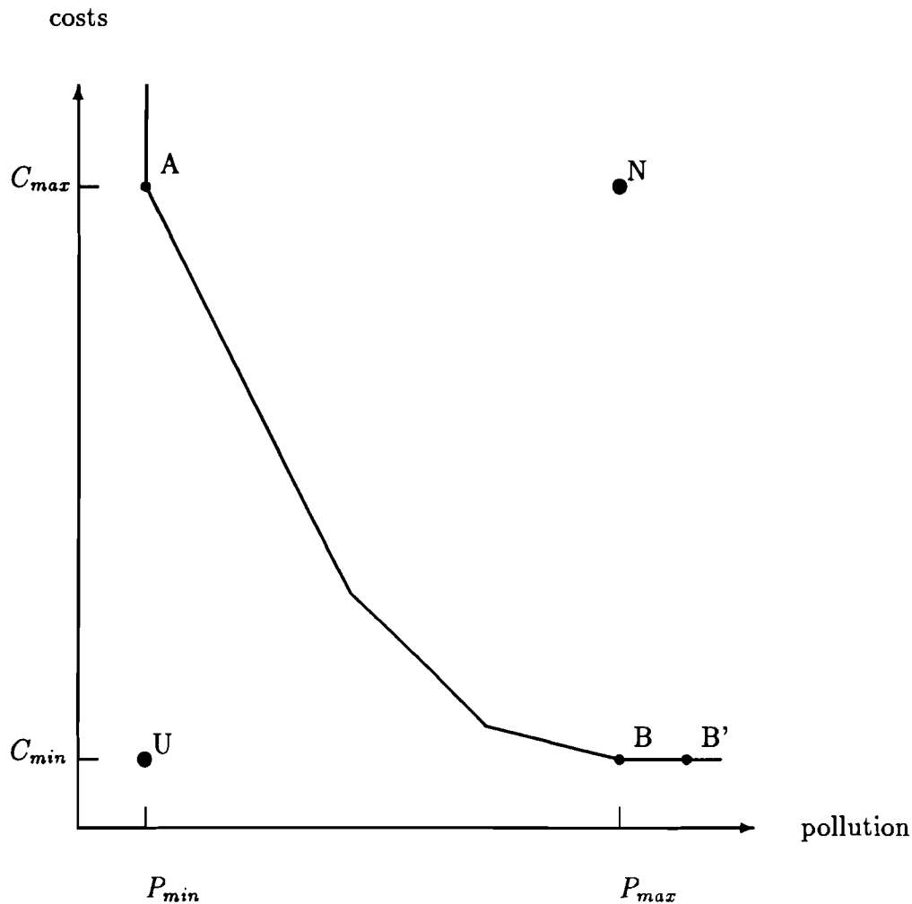
Figure 1: The illustration of the analysis of the Pareto surface.
