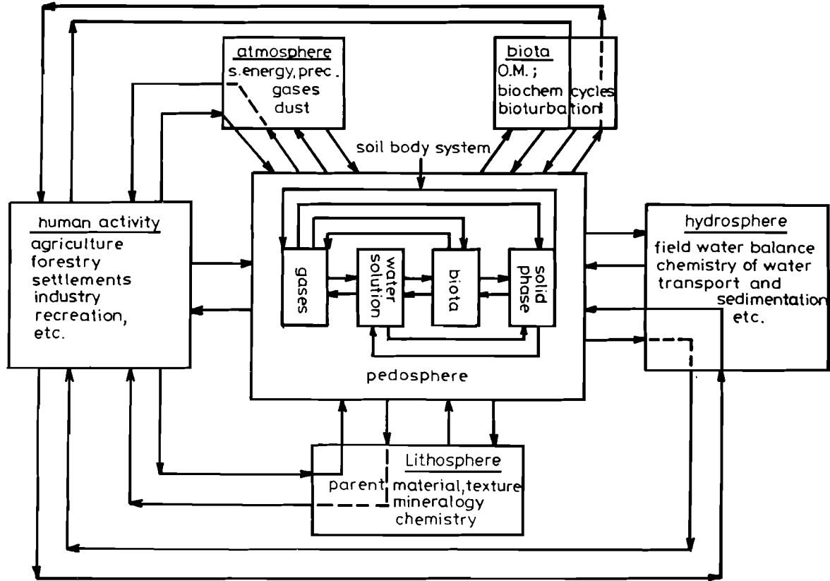
Figure 1. Model of the natural and human-induced interactions within the soil; and between soil and other bio-geospheric subsystems
