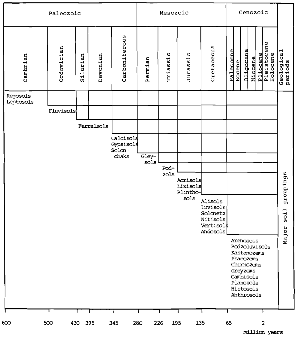
Figure 3. Evolution and diversification of the World's soil cover. /Tentative scheme/ /adapted from FRIDLAND and BUYANOVSKIY, 1977/
