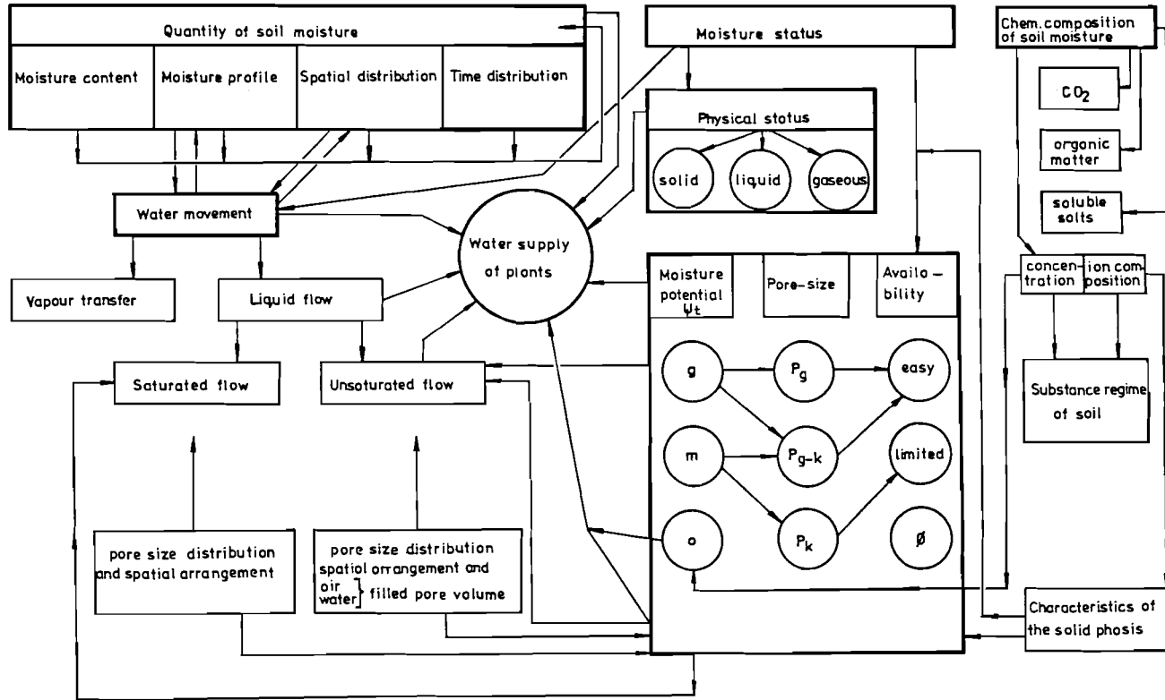
Figure 6. Main characteristics of soil moisture regime. g = gravitational potential; m = matric potential; o = osmotic potential; P_g = gravitational pore space; P_k = capillary pore space
