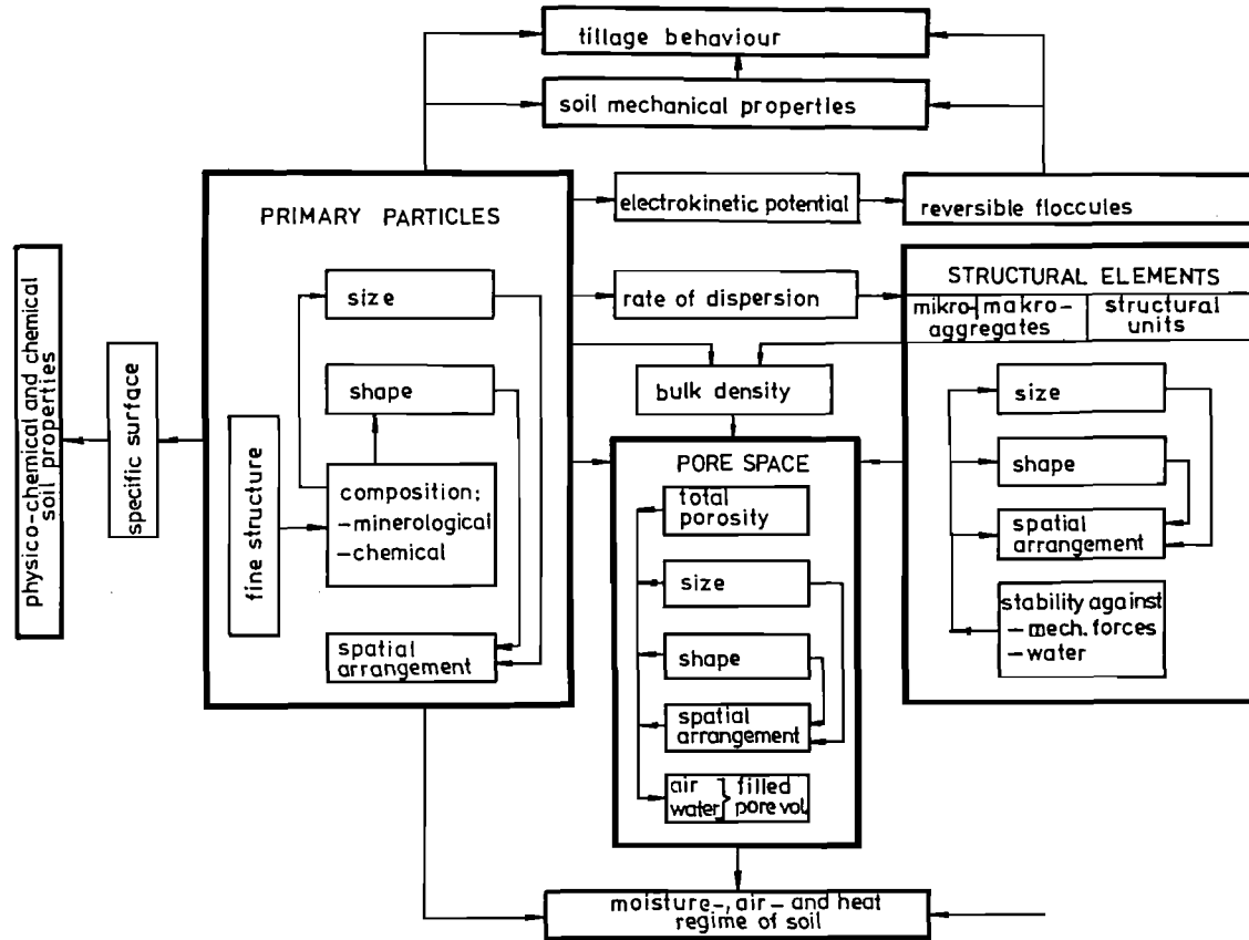
Figure 5. Characteristics of the solid phase of soil
