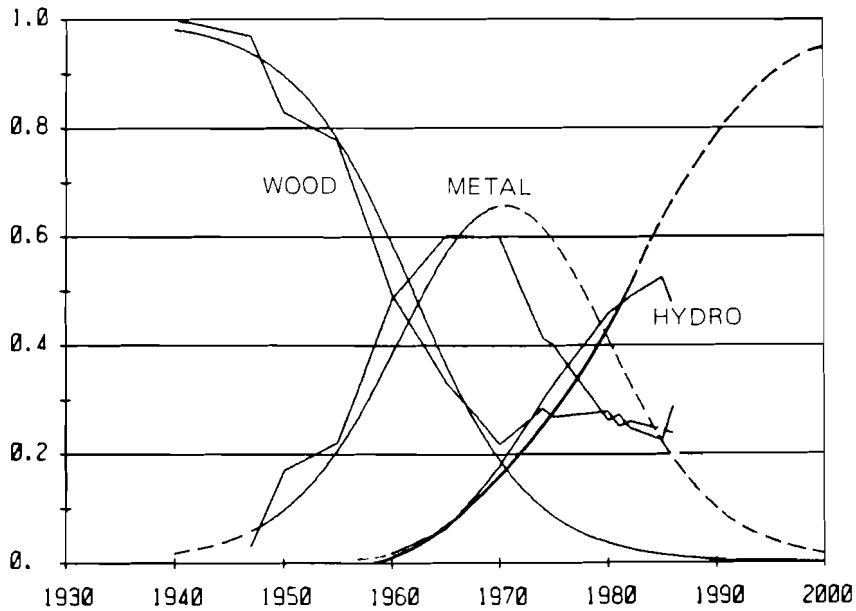
Figure 4A. Share of different roof supports in the total number of faces in the underground coal mining industry of the USSR (linear scale).
