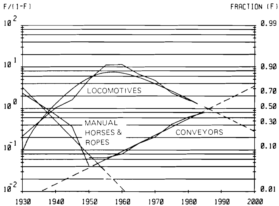
Figure 7B. Share of different transport modes at horizontal roads in underground coal mining industry of the USSR (logarithmic transformation).
