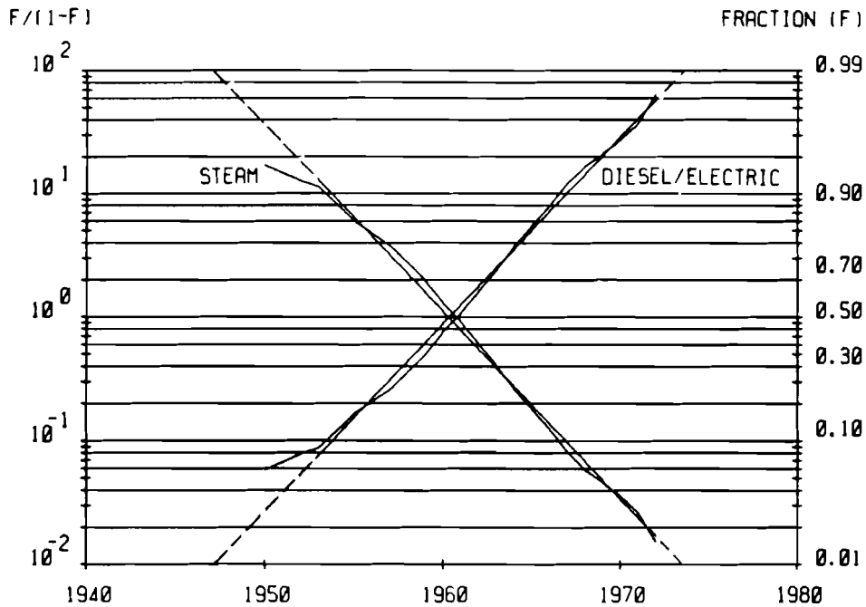
Figure 1B. Replacement of steam by diesel/electric locomotives, in fractional share of ton-km transported in the USSR (logarithmic transformation). Adapted from Kruglikov, 1985.
