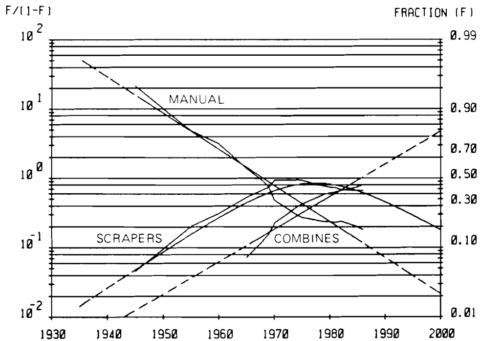
Figure 6B. Evolution of shares of different driving technologies in amount of driving work, total underground coal mining industry of the USSR (logarithmic transformation).
