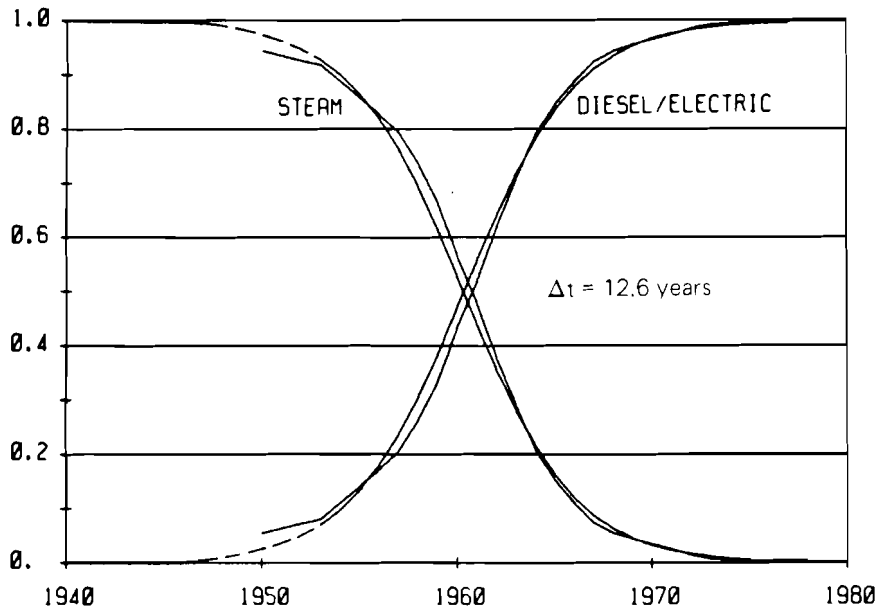
Figure 1A. Replacement of steam by diesel/electric locomotives, in fractional share of ton-km transported in the USSR (linear scale). Adapted from Kruglikov, 1985.
