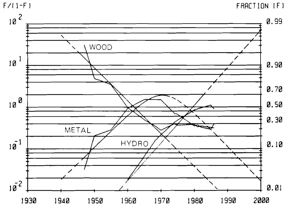
Figure 4B. Share of different roof supports in the total number of faces in the underground coal mining industry of the USSR (logarithmic transformation).
