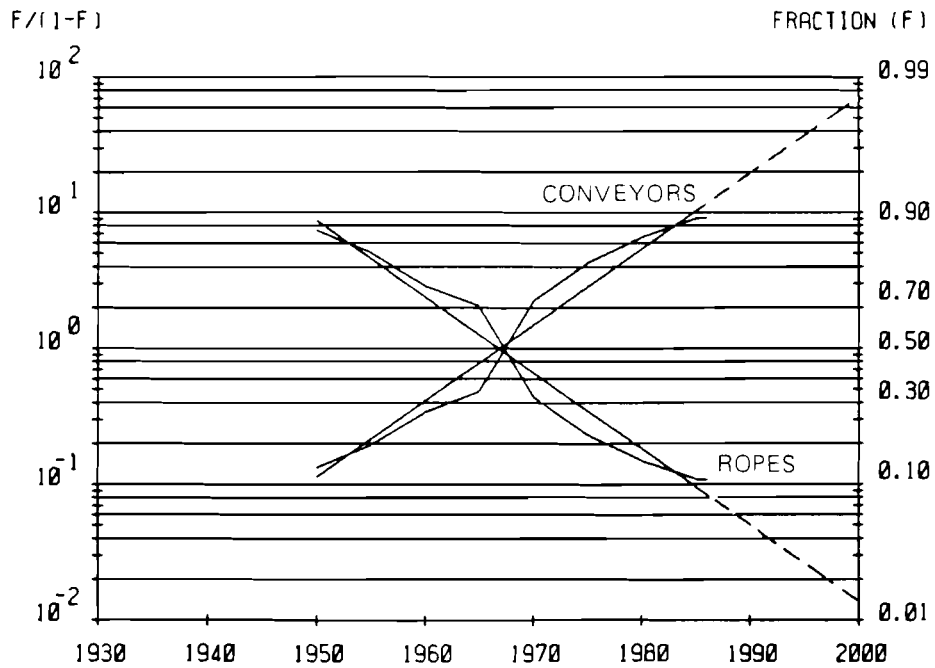
Figure 8B. Share of rope assets and conveyors at inclined workings in underground coal mining industry of the USSR (logarithmic transformation).
