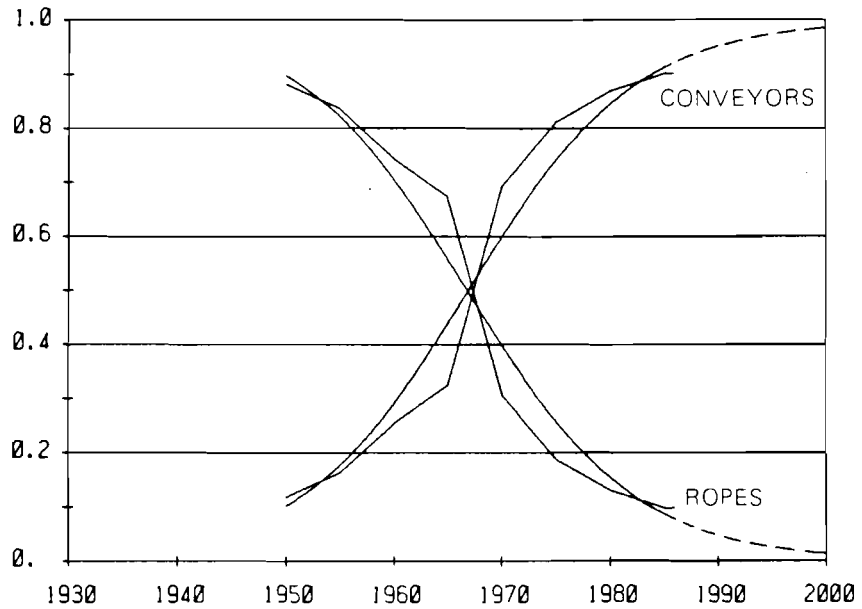
Figure 8A. Share of rope assets and conveyors at inclined workings in underground coal mining industry of the USSR (linear scale).
