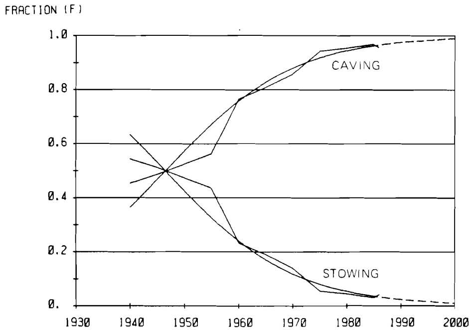
Figure 2A. Evolution of coal output by two main types of roof control in the Donbass (linear scale).
