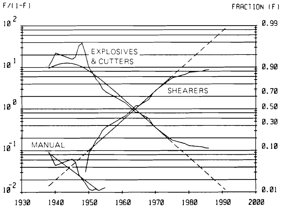
Figure 3B. Evolution of coal output by three technologies of coal winning at coal faces in the underground coal mining industry of the USSR (logarithmic transformation).
