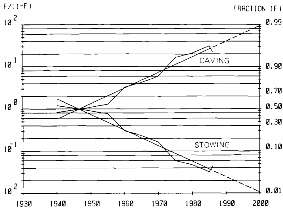
Figure 2B. Evolution of coal output by two main types of roof control in the Donbass (logarithmic transformation).
