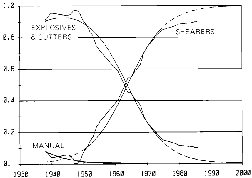
Figure 3A. Evolution of coal output by three technologies of coal winning at coal faces in the underground coal mining industry of the USSR (linear scale).
