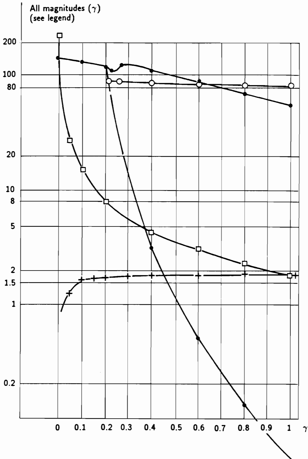
Figure 7: Some quantities of system (4.17) with various values of the parameter extinction coefficient \gamma . Two curves ( \bullet ) arising after \gamma \approx 0.22 is amplitude of the younger wave - meanings of n^{\max} = n(t, 100) and n^{\min} = n(t, r^{\min}) - see Figure 8. \circ - oscillation period \theta(\gamma) , \square - leaf area index \sigma(\gamma) in T = 2000 , + - value of J = \gamma \cdot \sigma(\gamma) .
