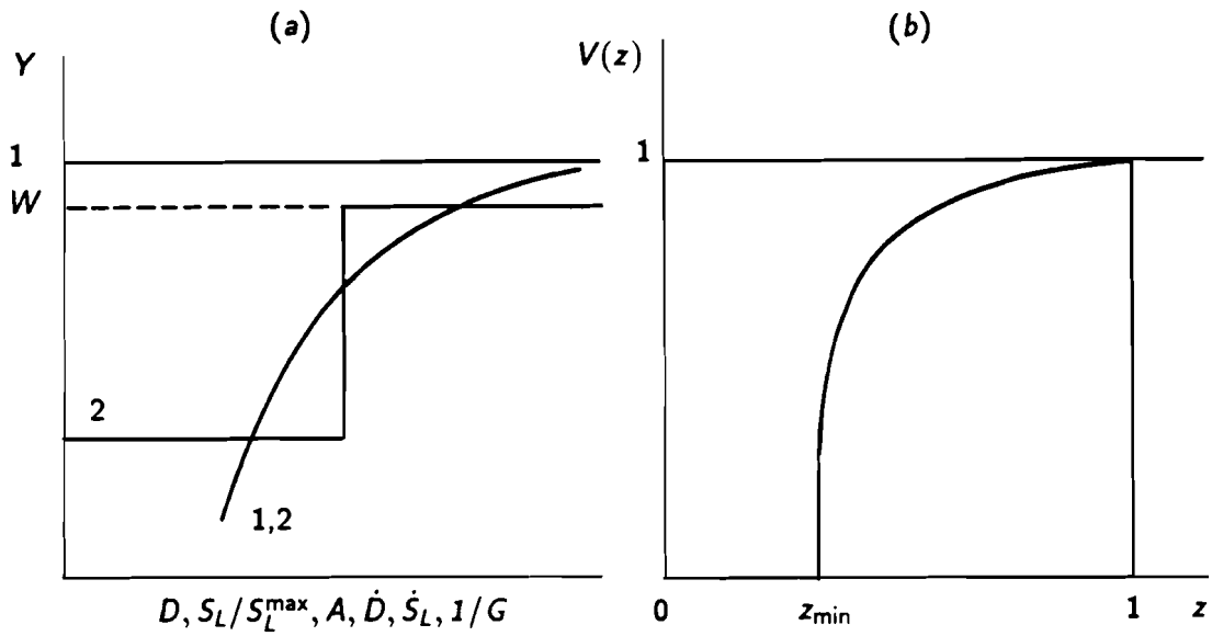
Figure 1: Qualitative behavior and arguments of viability function Y for a single tree. (a) empirical (1) and model (1, 2) forms following field data and model (see text for references and denotations). W - viability of mature, maximum defenced tree. (b) quality behavior of density-dependent viability components, V , on argument z = A/A_{\max} ; V is recommended for 'base model 1' (Section 3.3) and used in 'base model 2' (Section 4.3); z_{\min} = A_{\min}/A_{\max} where A_{\min} is maintenance respiration of leaves or whole tree.
