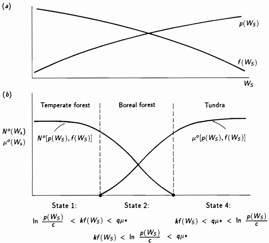
Figure 11: Parametric evolution in tree-moss system (5.5): if one considers p, f as monotone functions of soil moisture W_S – (a), then steady states of (5.5) – N^\circ(W_S), \mu^\circ(W_S) realize trajectories – (b), which can be interpreted as different types of tree-moss ecosystems disposed along environmental gradient (case of monotonous U(\mu) , consequence of states 1 \rightarrow 2 \rightarrow 4 ). Underneath Figure 11b we adduce the conditions of each state of realization in system (5.5).
