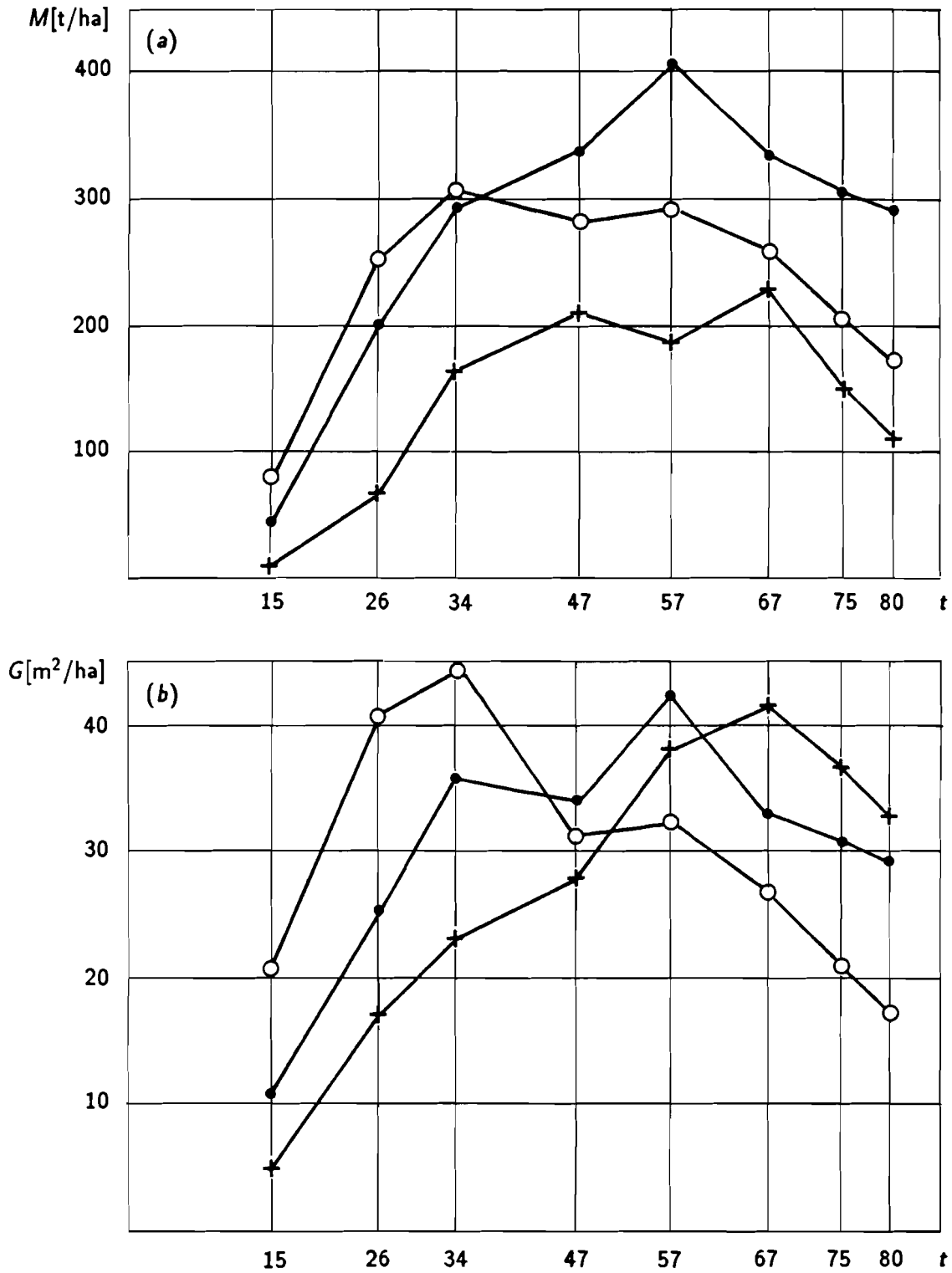
Figure 4: Trajectories of population biomass M - (a), and cross section area G - (b) (which is proportional to \sigma under initial densities N_1(o) = 1000 - (+), N_2(o) = 2400 - ( \bullet ), and N_3(o) = 10000 - o ); data from permanent plots with Pinus sibirica in Moscow region. "Overcrowding" effect consists of M_3^{\max} < M_2^{\max} under N_3(o) > N_2(o) , whereas all G_i^{\max} are approximately equal, only t_{G_i}^{\max} changes.
