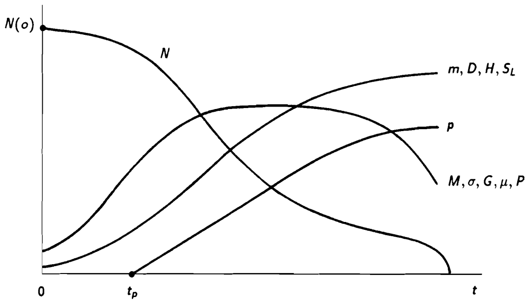
Figure 2: Qualitative dynamics of major variables of even-aged systems; curves with the same type of behavior are unified: \mu = mN^{3/2} (see text for denotations).
