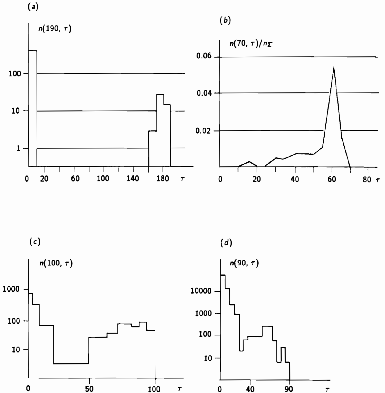
Figure 6: "Age waves" emerging after major forest cover disturbance in sufficiently dense stands. n(t, \tau) is the number of trees in age interval \Delta\tau = 1 under age \tau , t is moment of observation (equal to time since disturbance). Cases of strong suppression of juveniles by mature canopy: (a) - post fire succession, Pinus sibirica , West Siberia (Semetchkin 1970); (b) - post cutting succession, sum of oak, maple, and birch, New England (Oliver 1978). Cases of weak suppression: (c) - post fire succession, sum of spruce, Pinus sibirica , and fir, West Siberia (Korzukhin et al. 1988); (d) - post fire succession, mixed oak forest. Appalachian Mountains (Ross et al. 1982).
