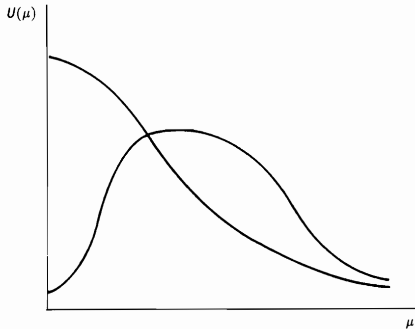
Figure 10: Qualitative dependence of seed survival and germination. U , on moss biomass; \mu (or thickness) for boreal tree species. a – small seeds (birch, spruce), b – large seeds, in particular Pinus sibirica , whose seed viability is maximal under a certain moss thickness (summarized in Katayeva and Korzukhin 1987).
