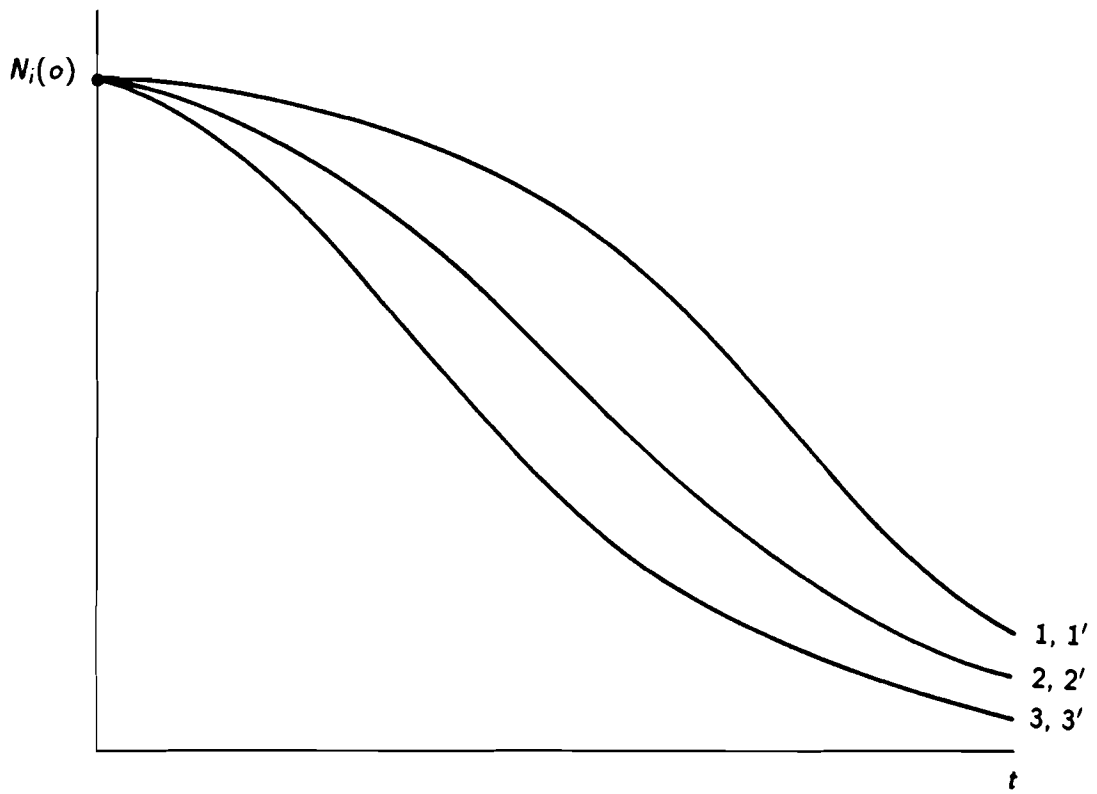
Figure 5: Given the equal initial numbers of trees, N_i(0) , N(t) falls rapidly for ameliorated site conditions ( 1 \rightarrow 2 \rightarrow 3 ) and with decreasing shade tolerance ( 1' \rightarrow 2' \rightarrow 3' ).
