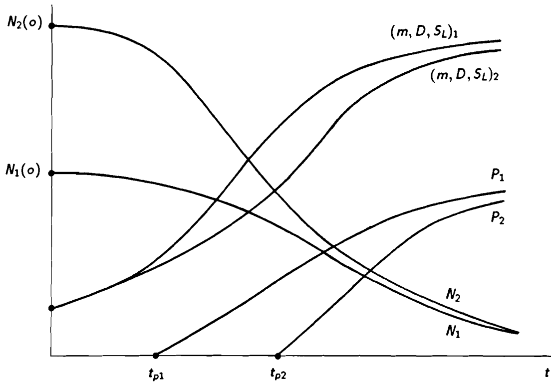
Figure 3: A set of even-aged system trajectories obtained under various initial densities (see text for denotations).
