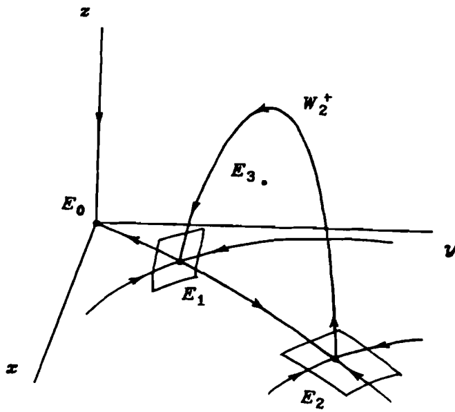
Figure 5. The separatrix cycle in system (1.1).
