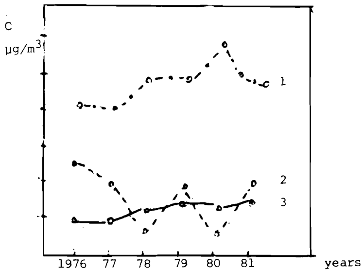
Borovoe, SO 2 , warm seasons
