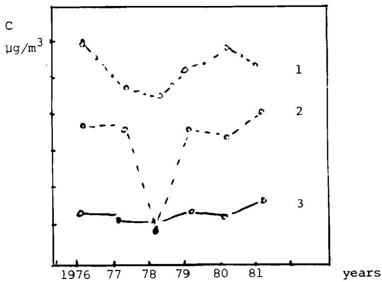
Borovoe, PB, cold seasons
