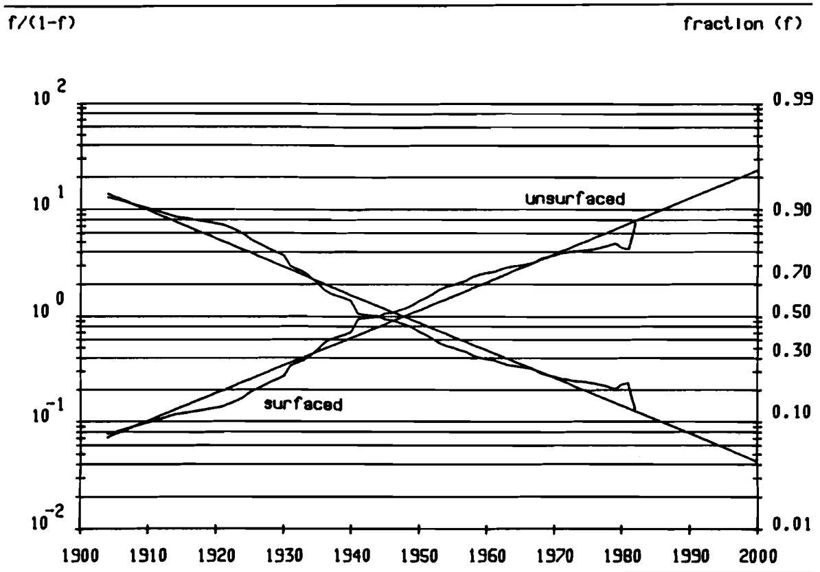
Figure 2.9 Substitution of Unsurfaced by Surfaced Roads, US.
