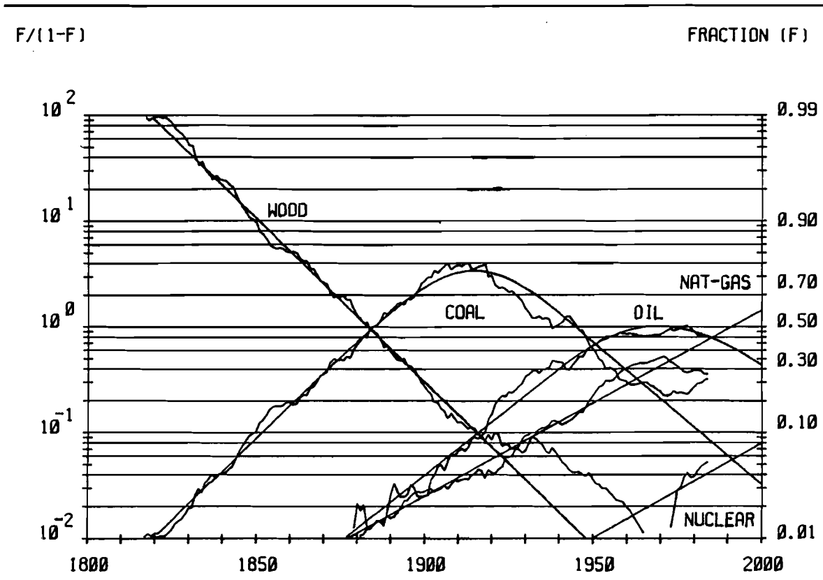
Figure 3.2 Primary Energy Substitution, US.
