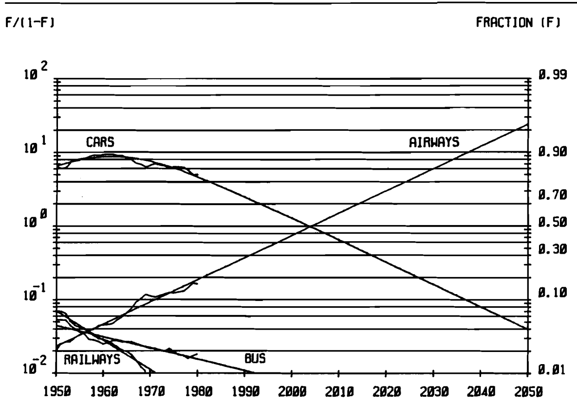
Figure 2.15 Intercity Passenger Traffic Substitution, US.
