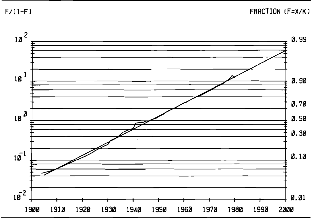
Figure 2.10 Mileage of Surfaced Roads, US.
