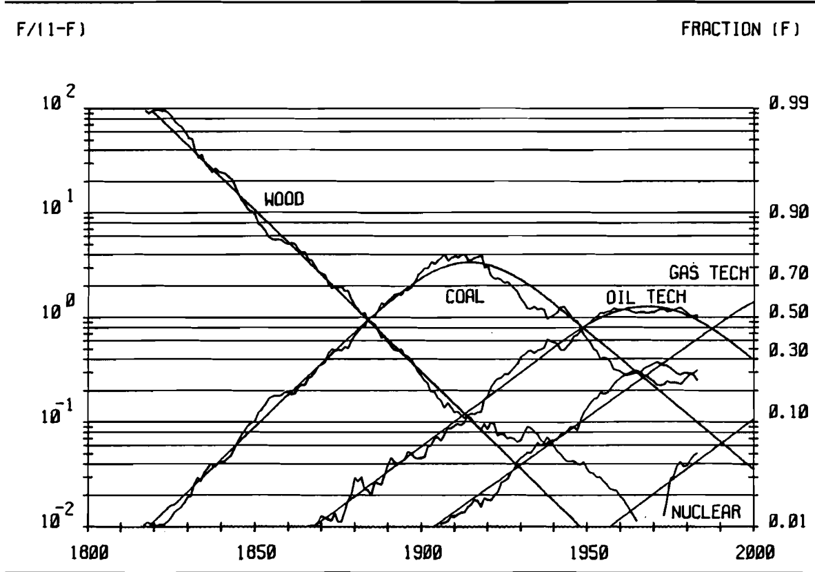
Figure 3.4 Energy Substitution and Gas Technologies, U.S.
