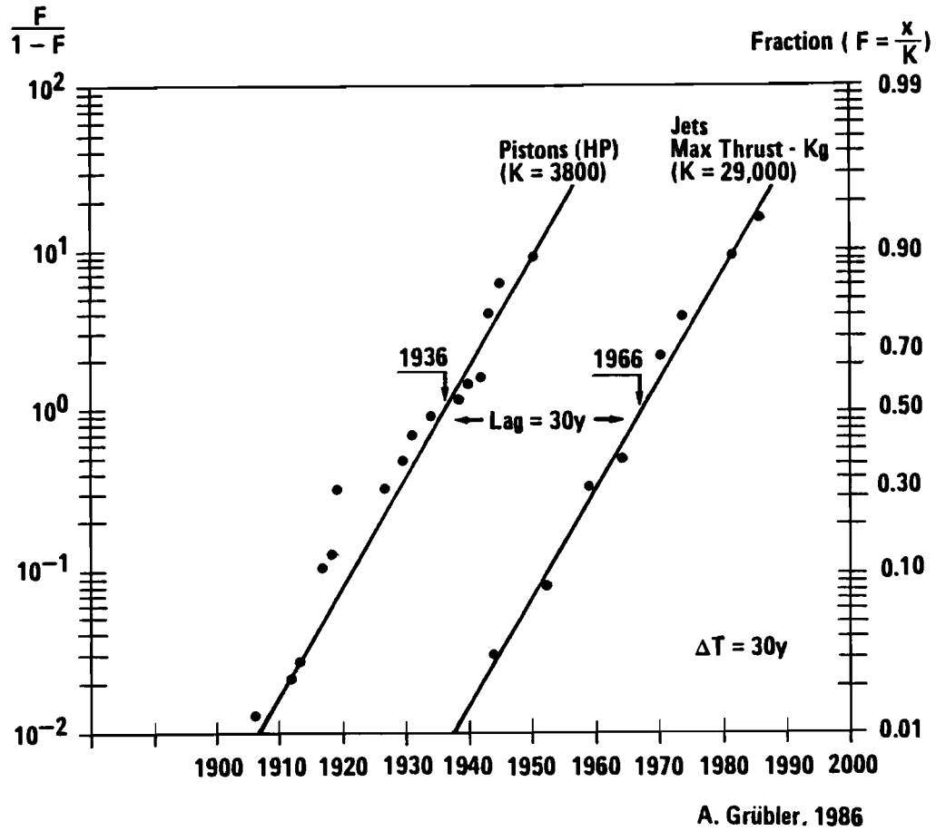
Figure 2.4 Performance of Aircraft Engines.
