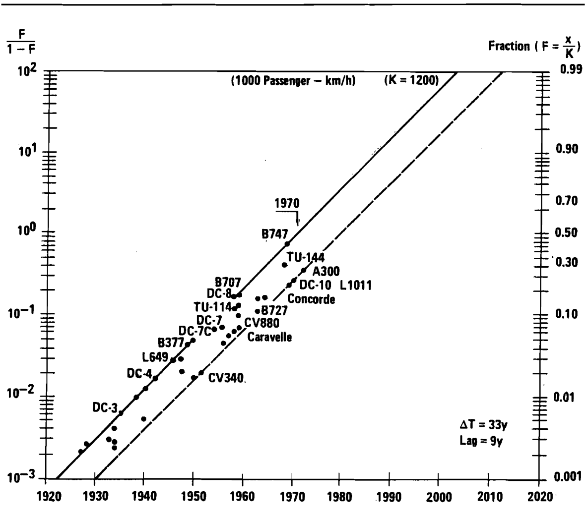
Figure 2.3 Passenger Aircraft Performance.
