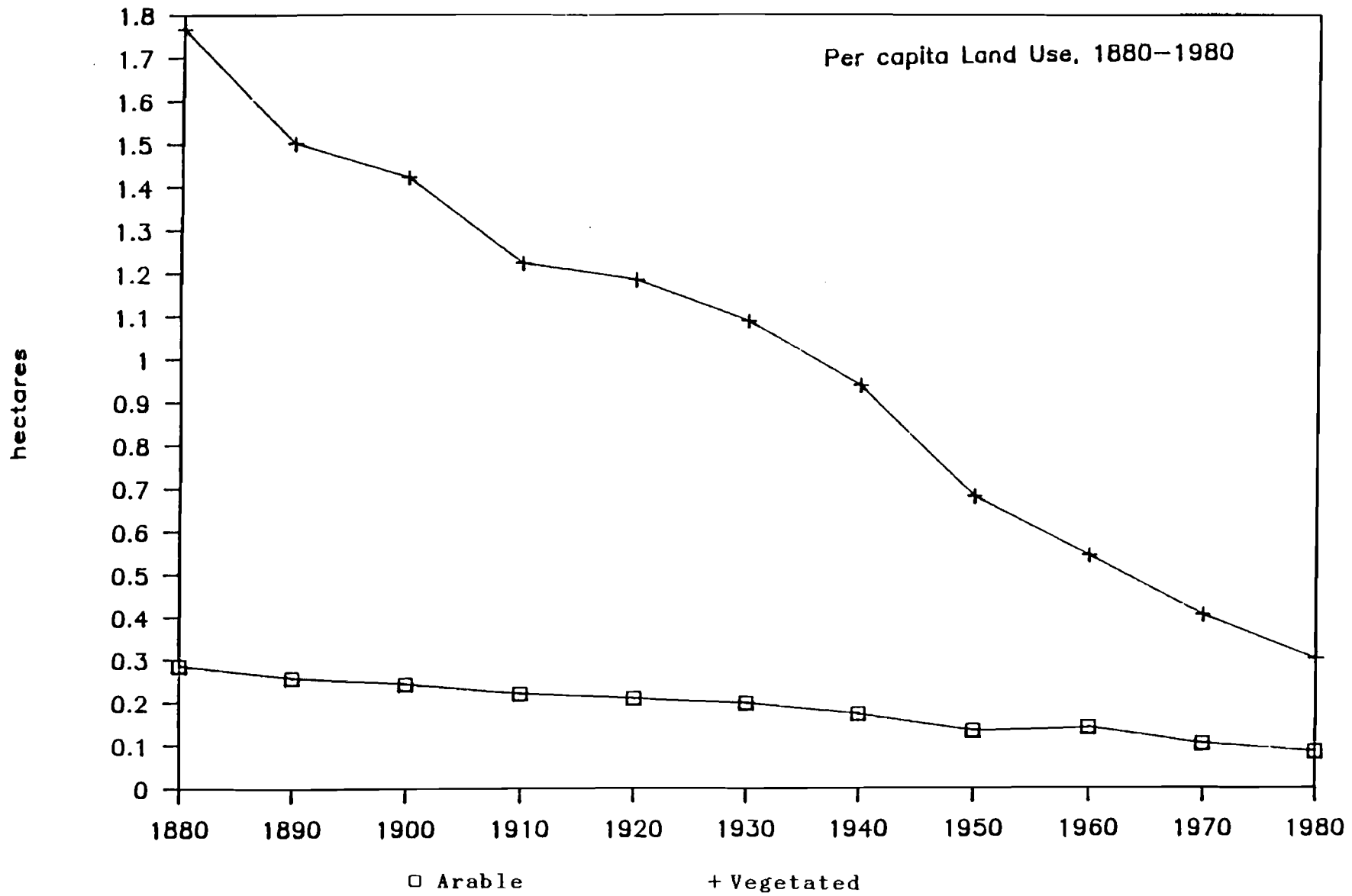
Fig. 5-4 The average area of arable land per person (lower curve); the average area of vegetated land per person (upper curve).
