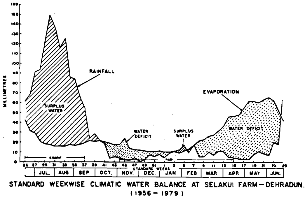
Figure 1 Annual water balance of the Doon valley, comparing precipitation and evaporation
