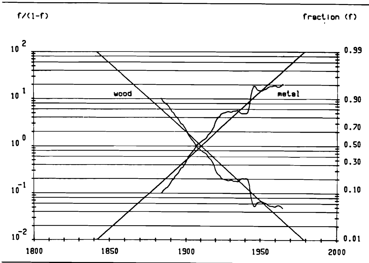
Figure 2.6 Substitution in Merchant Vessels by Structural Material.
