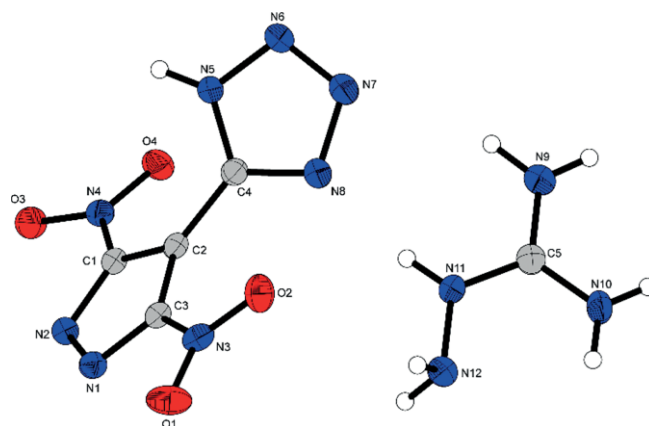
Figure 7. Molecular unit of compound 7 , showing the atom labeling scheme. Thermal ellipsoids represent the 50% probability level and hydrogen atoms are shown as small spheres of arbitrary radius.
