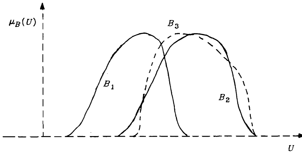
Figure 3. Three induced fuzzy sets (B_1, B_2, B_3) on U .
