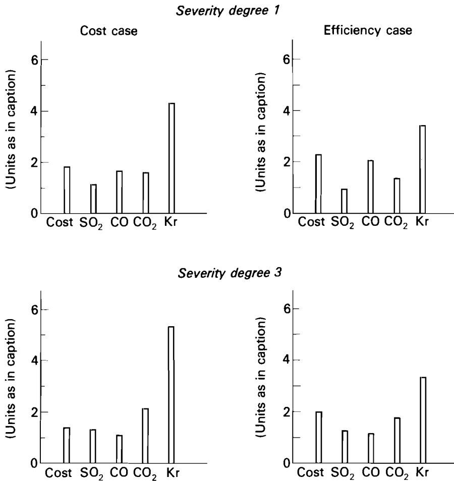
FIGURE 11 Total cost and principal emissions. The units used are as follows: total cost, 10^{11} Swiss Francs; \text{SO}_2 , 10^5 tonnes; CO, 10^5 tonnes; \text{CO}_2 , 10^7 tonnes; Kr, 10^4 Ci.
