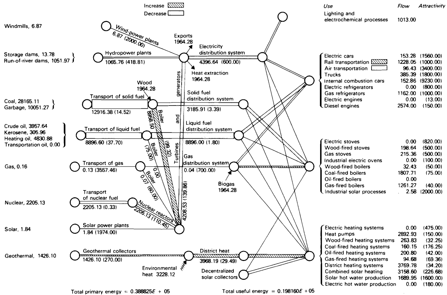
FIGURE 13 The energy-flow system for the cost-environment case. Units of MW are used throughout.
