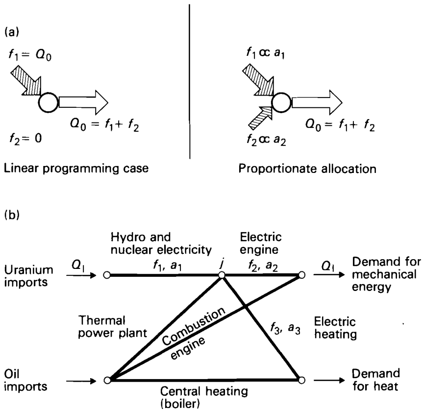
FIGURE 8 Proportionate allocation: (a) for two technologies, showing how it differs from linear programming; (b) for an energy system.
