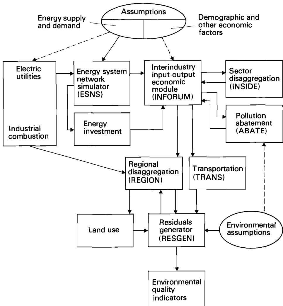
FIGURE A1.1 A block diagram of SEAS.
