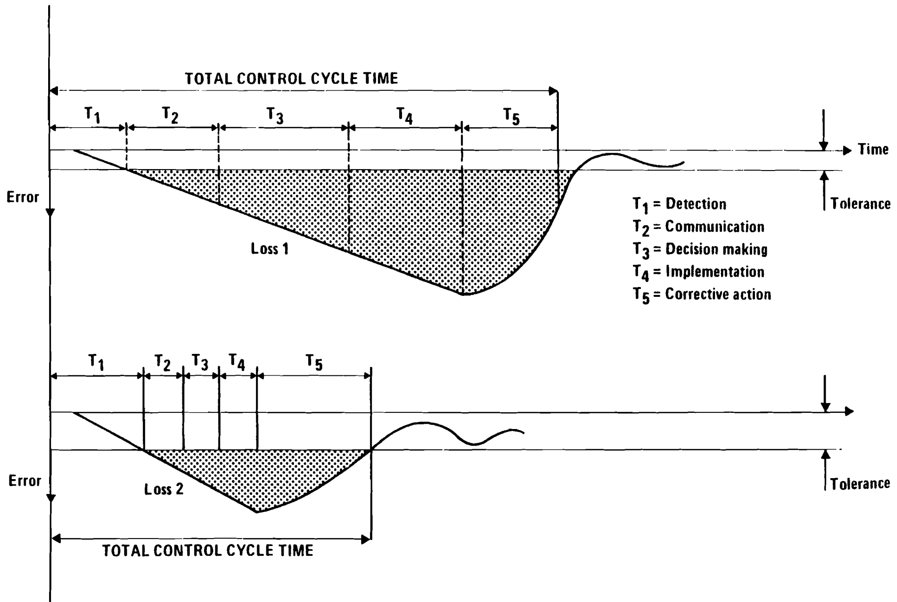
Figure 11. Real-time total mill information and control system can remarkably shorten the total cycle time thus improving profitability. (Uronen 1979)
