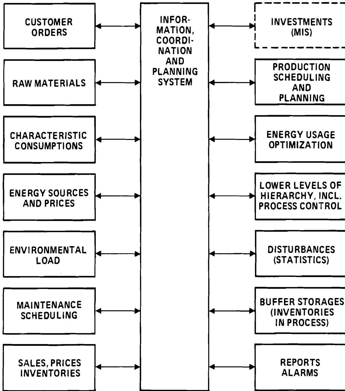
Figure 8. Tasks of total mill information and production planning system.
