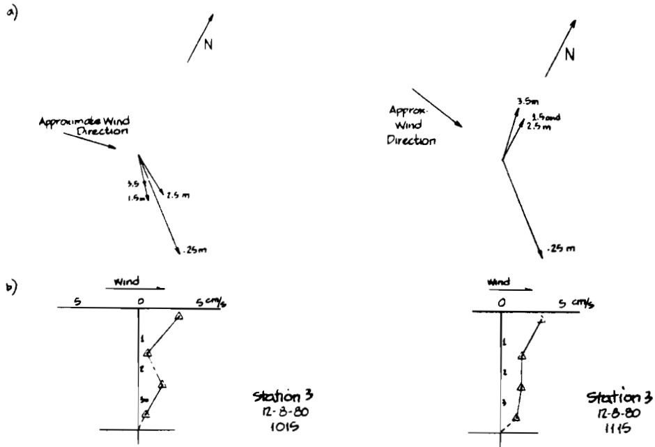
Figure A.10 Current Measurements at Station 3, 12 August 1980
