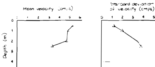
Figure A.9 Temporal statistics of continuous measurements at Station 1 11 August 1980
