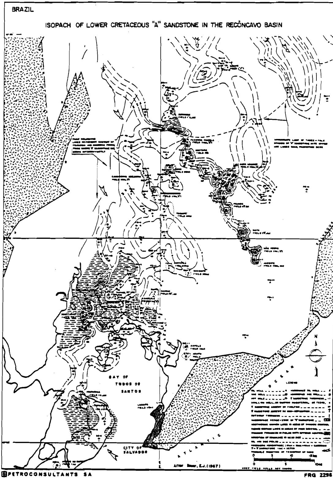
FIGURE 6. ISOPACH OF LOWER CRETACEOUS "A" SANDSTONE IN THE RECONCAVO BASIN.
