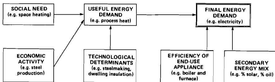
Figure 1. Determinants of useful and final energy demand.
