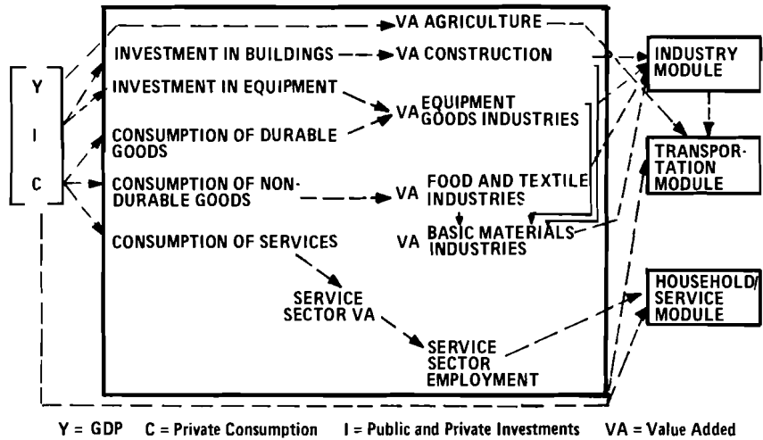
Figure 5. Macroeconomic module of MEED 2*.
