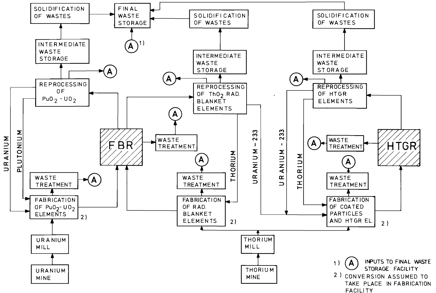
FIGURE 2.1 ASYMPTOTIC NUCLEAR FUEL CYCLE
