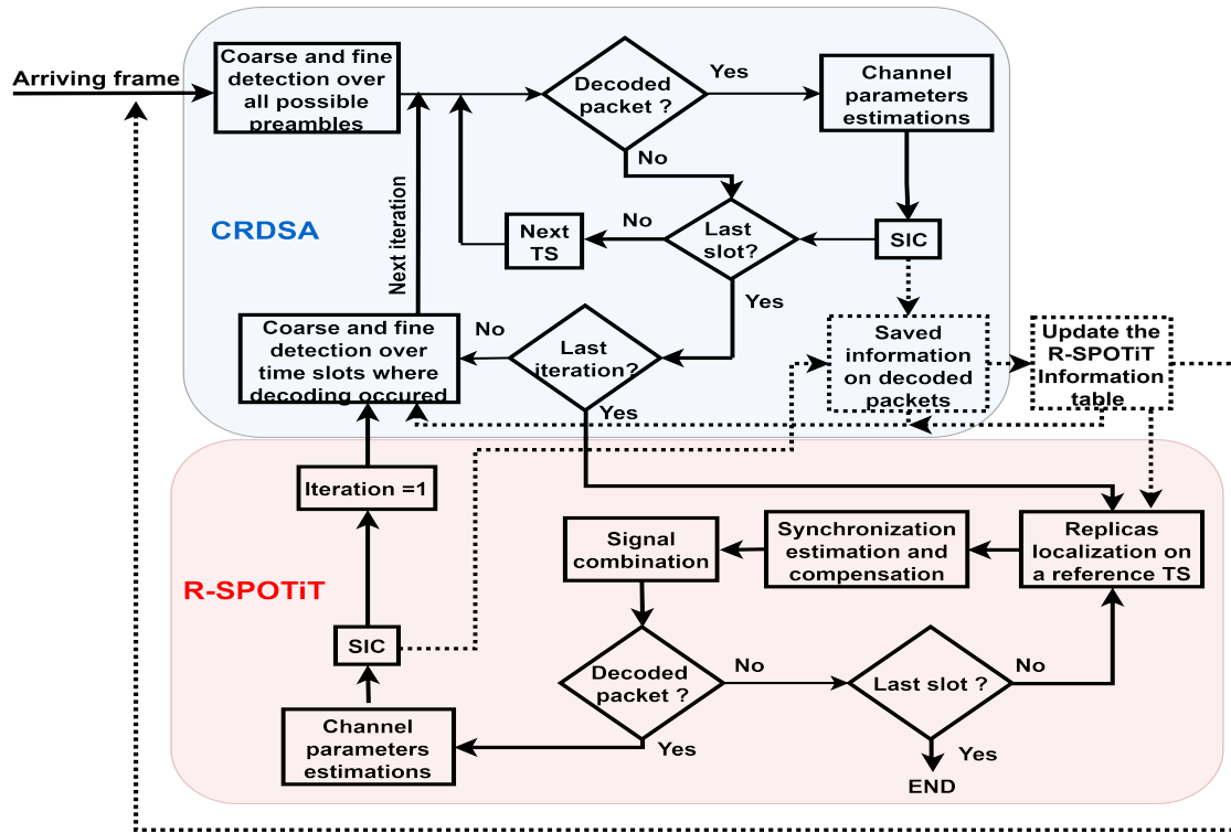
FIGURE 5 Detailed overview of the receiver.
