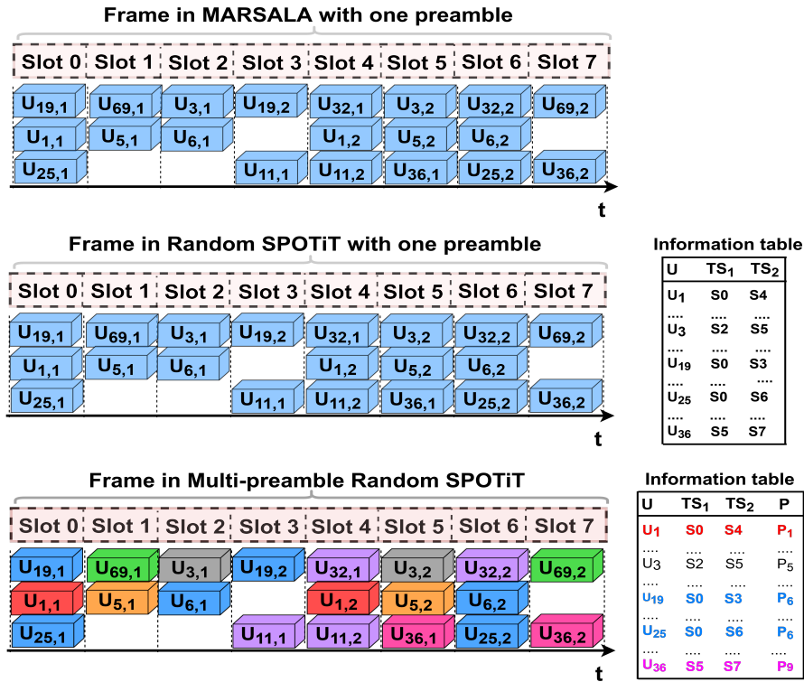
FIGURE 3 Frame structure example at reception.
