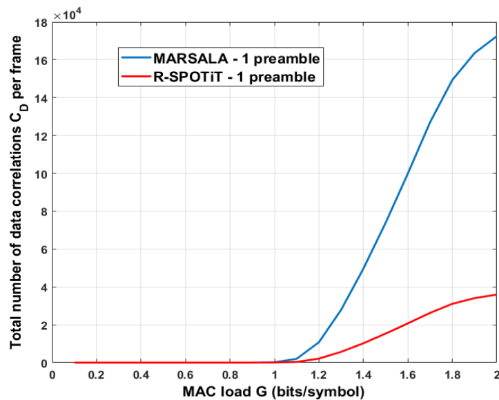
FIGURE 8 Data detection complexity in case of MARSALA and single preamble R-SPOTiT
