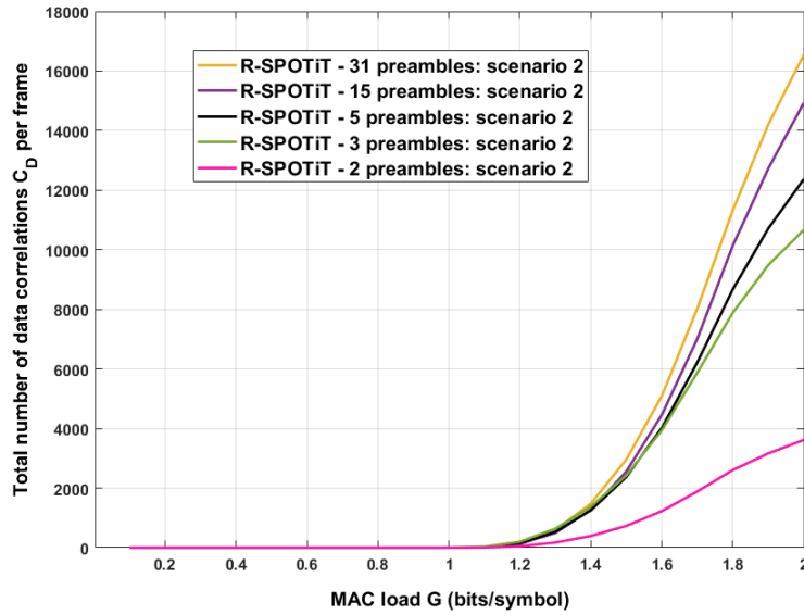
FIGURE 10 Data detection complexity in case of multi-preamble R-SPOTiT
