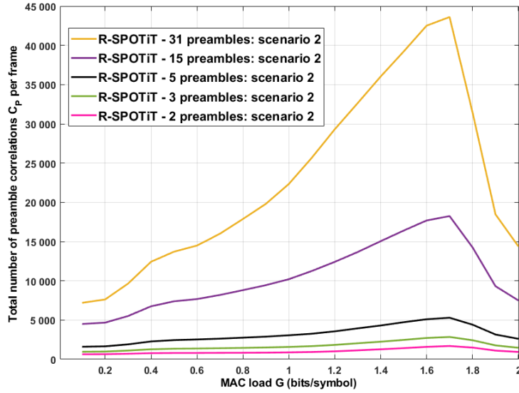
FIGURE 9 Preamble localization complexity in of case multi-preamble R-SPOTiT
