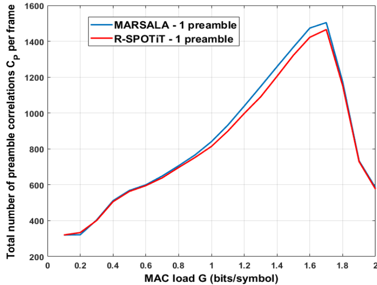
FIGURE 7 Preamble localization complexity in case of MARSALA and single preamble R-SPOTiT
