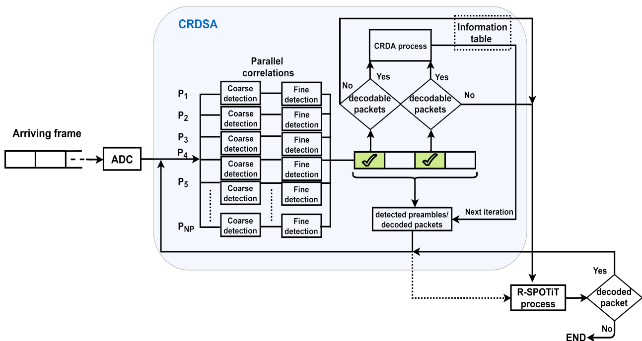
FIGURE 4 General overview of the receiver.
