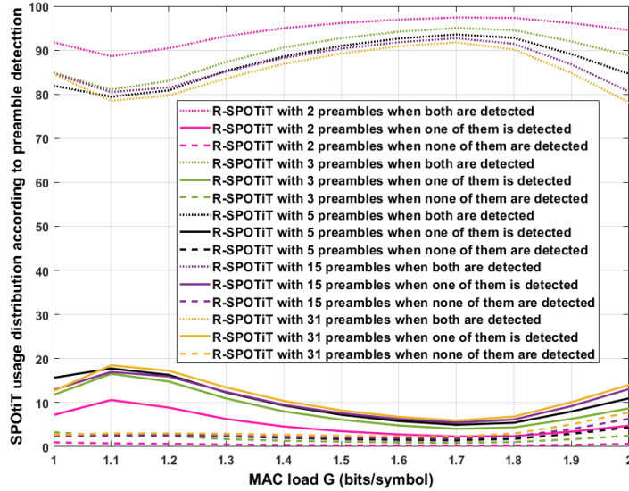
FIGURE 11 R-SPOTiT usage distribution, with N_{bt} = 16 and R = 5 per frame in percentage.
