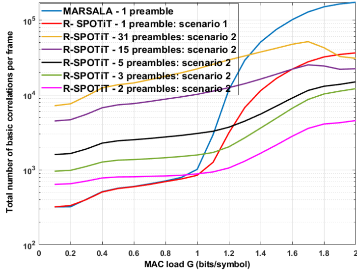
FIGURE 6 Overall frame complexity, with N_{bt} = 16 and R = 5 in CRDSA/MARSALA and CRDSA/R-SPOTiT environments
