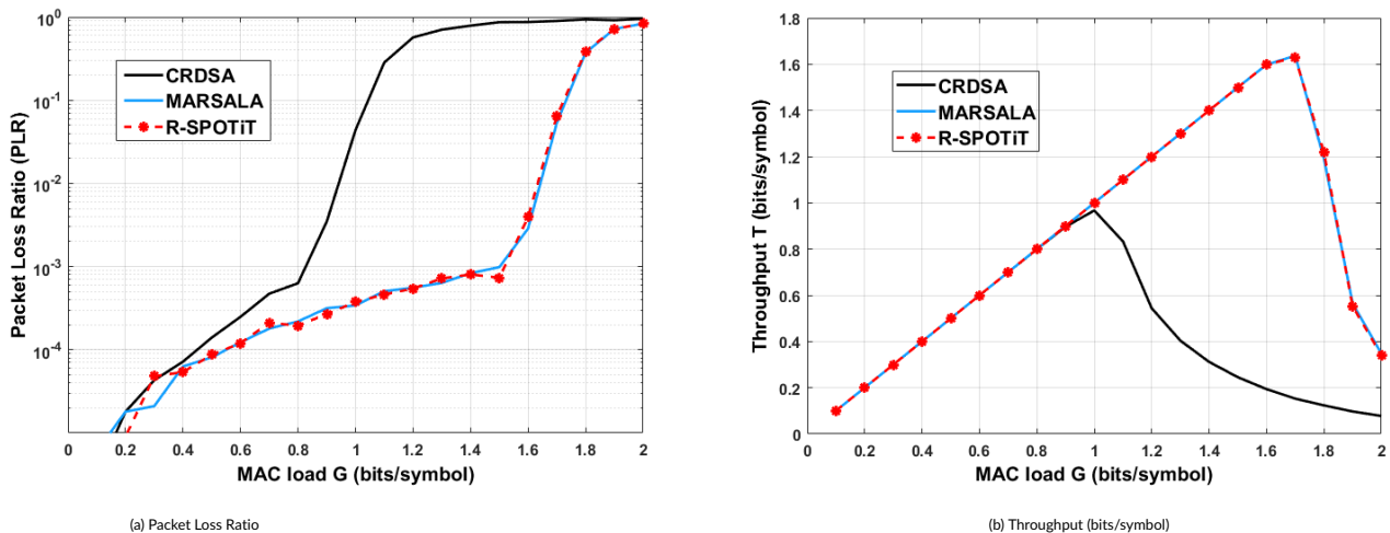
FIGURE 2 R-SPOTIT, MARSALA and CRDSA performance, 100 information bits, QPSK modulation, Turbo code of rate 1/3 , 100 slots per frame, AWGN channel and E_S/N_0 = 10 dB .
