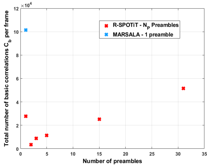
FIGURE 12 Overall frame complexity, with N_{bt} = 16 and R = 5 in CRDSA/MARSALA and CRDSA/R-SPOTiT with different numbers of preambles, for a channel load of 1.6 bits/symbol.
