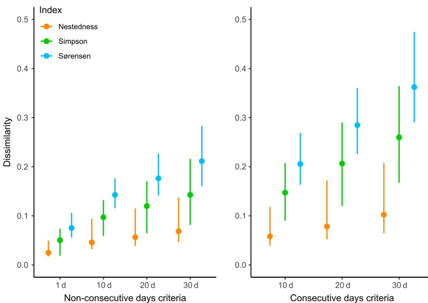
FIGURE 4 Community dissimilarity indices (average of pairwise nestedness, Simpsons species turnover, and Sørensen's total dissimilarity; see Methods) among sites for wetland birds during the 2014 breeding season (April–June), as a function of number of time units (1, 10, 20, and 30 days) in nonconsecutive (left) and consecutive (right) sequences required for inclusion of a species in local species lists
