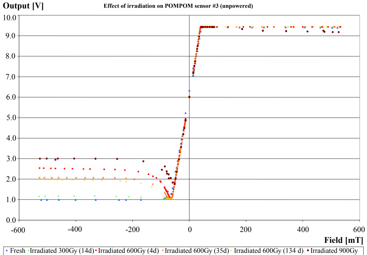
Figure 3: Effect of successive 300 Gy irradiations ( 60 Co) on sensor #3. Intervals between exposure and measurement are given in days, where relevant. The immediate effects of the second dose (to 600 Gy) abate within a few weeks, but the remaining damage lasts for months. The final (900 Gy) results were taken just a few hours after the irradiation; the scatter is from the real changes in device response with time as it recovers.
