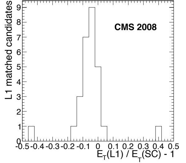
Figure 21: Level-1 e/\gamma E_T resolution for E_T(L1) > 10 GeV. The non-zero mean results from a combination of factors and is compatible with the LSB of E_T(L1) .
