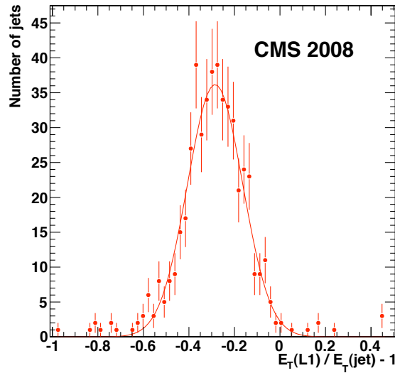
Figure 24: The E_T resolution of L1 jets.
