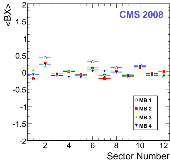
Figure 3: Mean BX from DT chambers of wheel 0.
