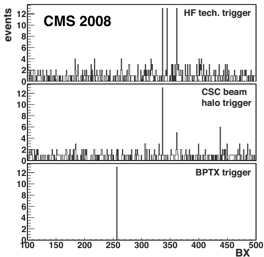
Figure 8: Measurement of the time delay in BX between the BPTX trigger and previously synchronised CSC beam halo and HF triggers, using beam splash events.
