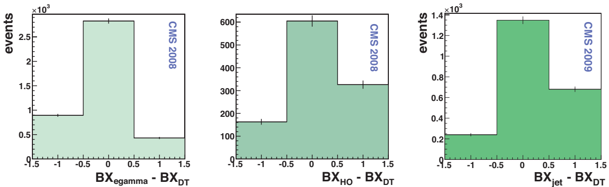
Figure 7: Time differences at the GT input between e/\gamma triggers (left), HO technical triggers (middle), and jet triggers (right, 2009 data), with respect to L1 muon candidates from the DT system.
