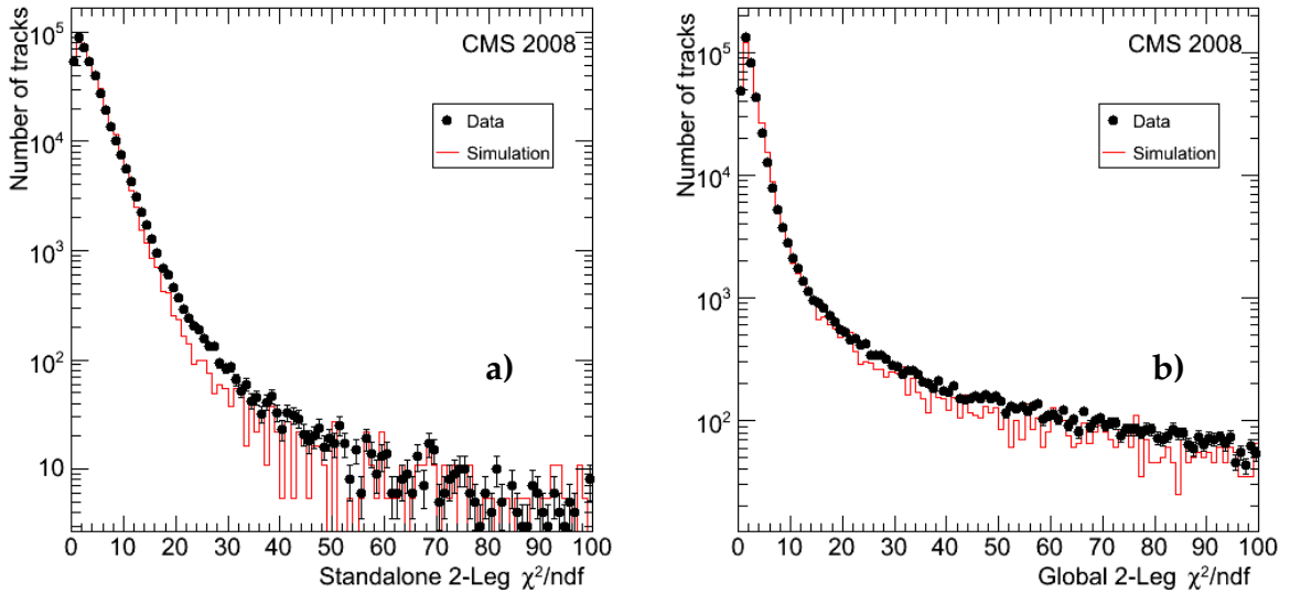
Figure 4: Distributions of the \chi^2/ndf of the track fit for the data (points) and for the Monte Carlo simulation (histogram), for a) CosmicSTA standalone muons and b) 2-leg global muons. The MC distributions are normalized to the number of events in the data.
