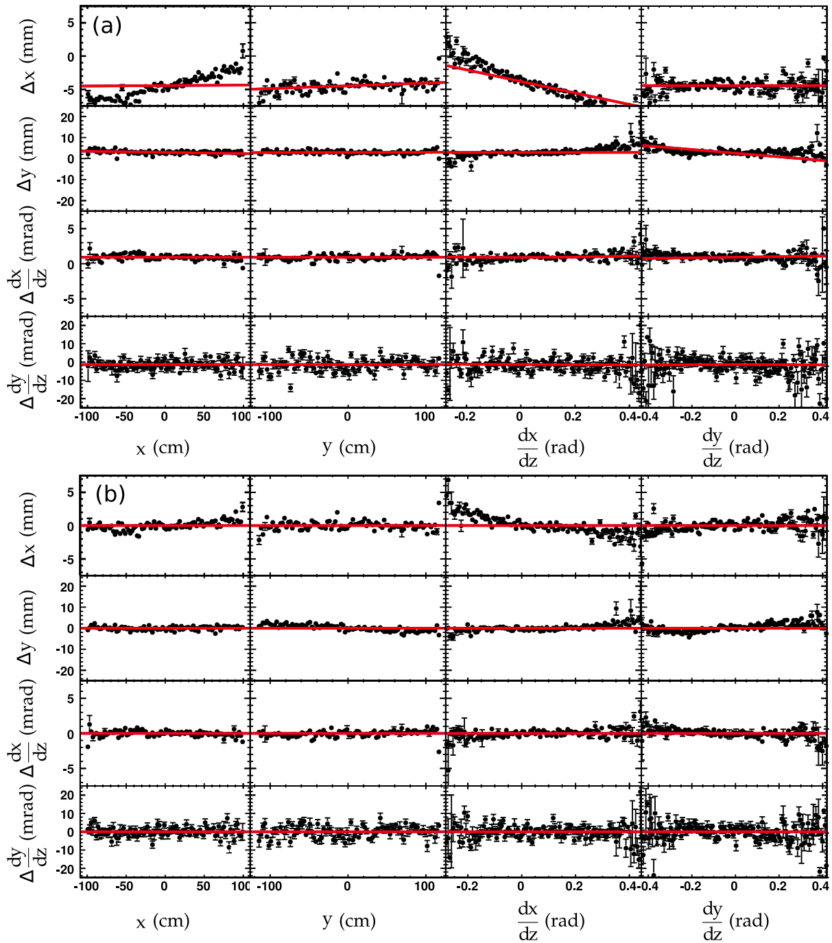
Figure 6: Mean residuals with statistical error bars versus position (x, y) and entrance angle (\frac{dx}{dz}, \frac{dy}{dz}) in one chamber (DT wheel 0, station 1, sector 10) from cosmic-ray data, (a) before alignment and (b) after alignment. Each bin selects a narrow range of the position or entrance angle component under consideration, but averages over all other variables. The fit function, evaluated at zero in all other variables, is overlaid as lines before and after alignment. Asymmetries in the position and entrance angle distributions allow for misalignments to be manifested in more ways in the averaged residuals than in the projections of the best-fit function, but the fit properly removes these misalignments, resulting in nearly flat lines in all variables.
