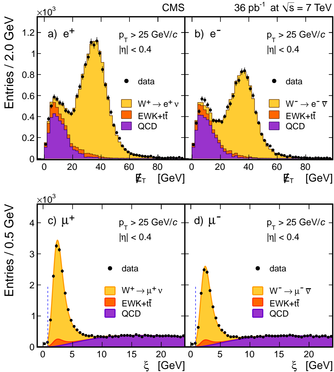
Figure 1: Signal fit to data \cancel{E}_T distributions for electrons, a) W^+ \rightarrow e^+ \nu , b) W^- \rightarrow e^- \bar{\nu} , and fit to \xi distributions for muons, c) W^+ \rightarrow \mu^+ \nu , and d) W^- \rightarrow \mu^- \bar{\nu} . Only the results for the first pseudorapidity bin ( |\eta| < 0.4 ) are shown. In Figs. c) and d), only events on the right of the dashed vertical line are included in the fit. The QCD (multijet and photon+jet production) shape is determined directly from data.
