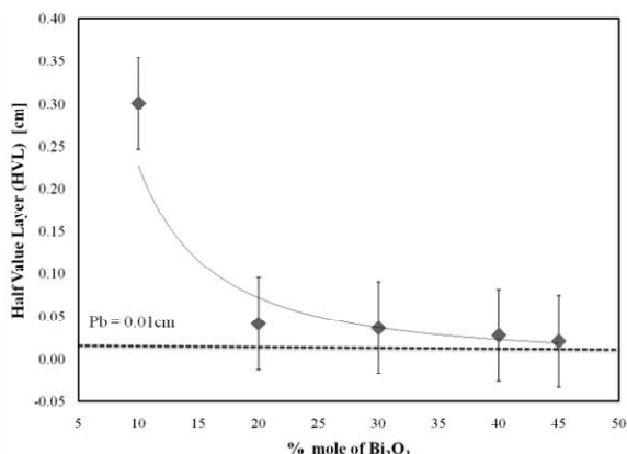
Figure 6: The Half Value Layer (HVL) of xBi 2 O 3 - (1-x)ZnO - 0.2B 2 O 3 - 0.3(SiO 2 )RHA glass samples compared to given value of Pb (0.01cm) using XCOM prediction program.
