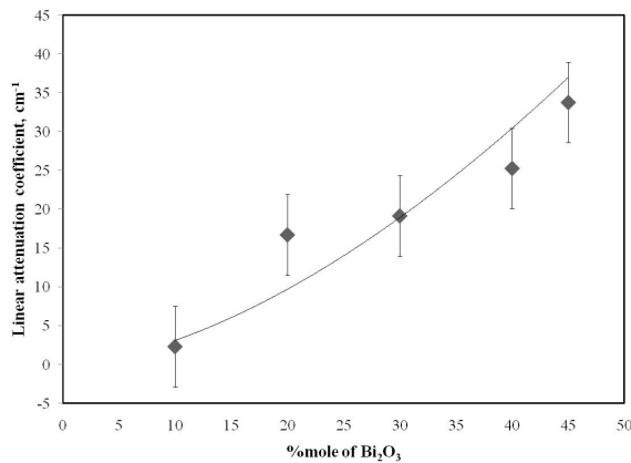
Figure 4: Linear attenuation coefficient of xBi 2 O 3 - (1-x)ZnO - 0.2B 2 O 3 - 0.3(SiO 2 )RHA glass samples.
