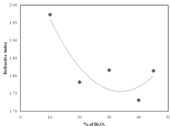
Figure 7: Refractive indices of xBi 2 O 3 - (1-x)ZnO - 0.2B 2 O 3 - 0.3(SiO 2 )RHA glass samples.
