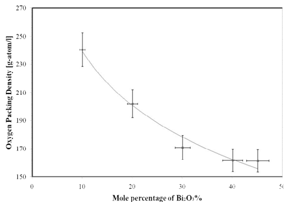
Figure 3: Oxygen Packing Density of xBi 2 O 3 - (1-x)ZnO - 0.2B 2 O 3 - 0.3(SiO 2 )RHA glass samples.
