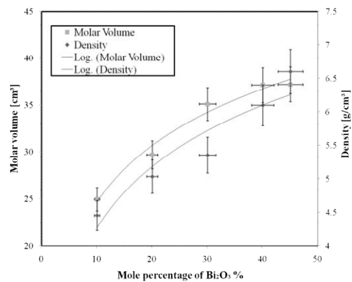
Figure 2: Molar Volume and Density of xBi 2 O 3 - (1-x)ZnO - 0.2B 2 O 3 - 0.3(SiO 2 )RHA glass samples.
