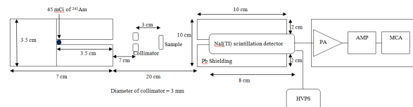
Figure 1: 241 Am gamma ray scattering experimental setup.
