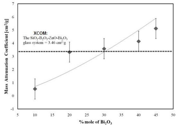
Figure 5: Mass attenuation coefficient of xBi 2 O 3 - (1-x)ZnO - 0.2B 2 O 3 - 0.3(SiO 2 )RHA glass samples compared to given value (3.46 cm 2 /g using XCOM prediction program.
