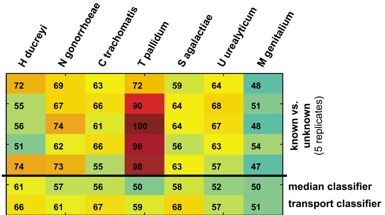
Figure 2 Discrimination between proteins of known and unknown function. The results of five random splits of test and training set are shown, and for comparison the lower two rows show the median performance of the function prediction classifier and the 'transport and binding' classifier for each species. For each species, except M. genitalium the average performance on the known-vs.-unknown task is better than on the function prediction task. In the case of T. pallidum , known and unknown proteins can be distinguished with almost perfect performance.
