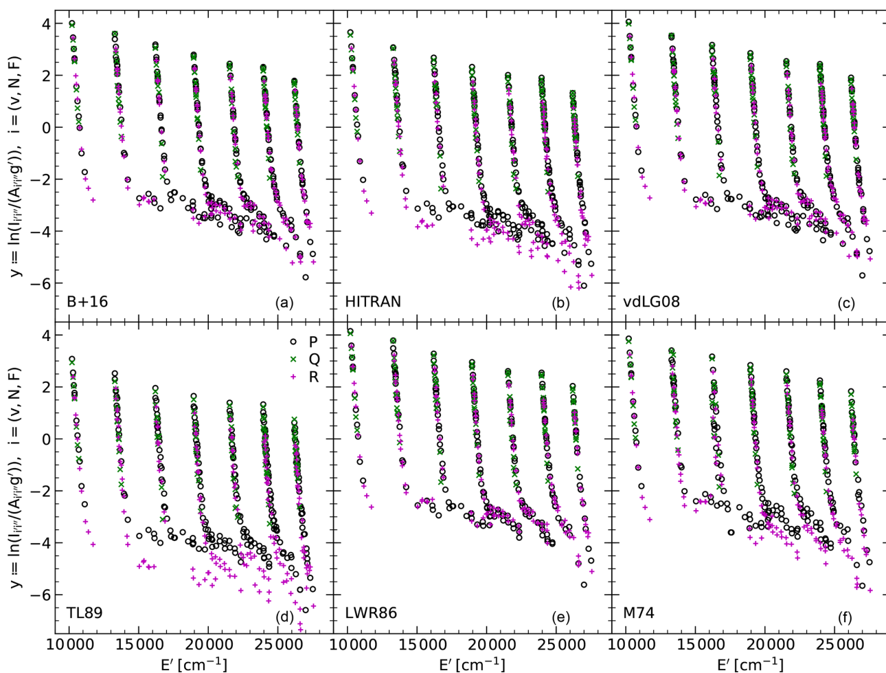
Figure 5. Distribution of logarithmic OH level populations y , i.e. line intensity in rayleighs divided by Einstein- A coefficient in inverse seconds and the statistical weight of the upper-level g' as a function of the upper-level energy E' in inverse centimetres. The six panels show the results for the reliable \Lambda -doublet measurements (see Fig. 2) neglecting OH(7-1) (two lines) for different sets of Einstein- A coefficients: Brooke et al. (2016) (B+16), HITRAN (Rothman et al., 2013), van der Loo and Groenenboom (2008) (vdLG08), Turnbull and Lowe (1989) (TL89), Langhoff et al. (1986) (LWR86), and Mies (1974) (M74). The number of plotted data points is smaller for older sets due to their limitations in the coverage of faint bands and high rotational levels. The populations derived from different branches ( P , Q , and R ) are highlighted by different symbols and colours (see the legend in d).
