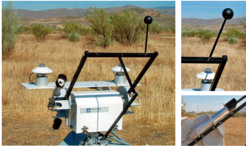
Figure 2.3: DLR reference measurement system for RSI calibration. Upper right: pyranometer with shadow ball. Lower right: pyrheliometer. [Quaschnig, 2011]
