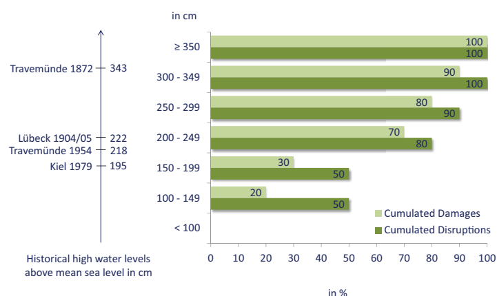
Figure 3: Critical amount of high water level for German Baltic sea ports
