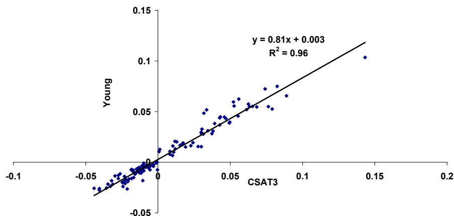
Fig. 8: Comparison of the buoyancy flux in \text{K}\cdot\text{m/s}
