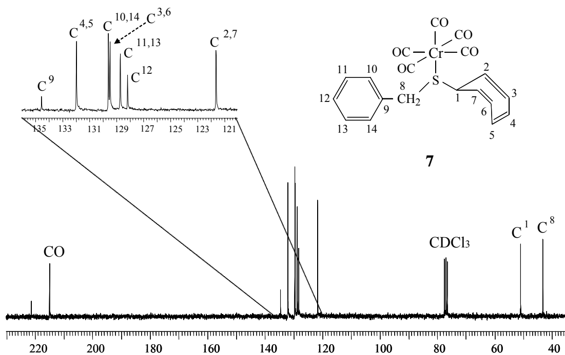
Fig.10. ^{13}C NMR Spectrum of Cr(CO)_5[PhCH_2S(C_7H_7)] ( 7 ) (in CDCl_3 at 25 °C)
