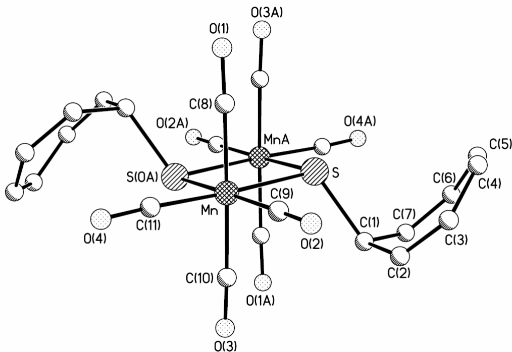
Fig.21. Structure of \text{Mn}_2(\text{CO})_8[\mu\text{-S}(\text{C}_7\text{H}_7)]_2 ( 17 )
