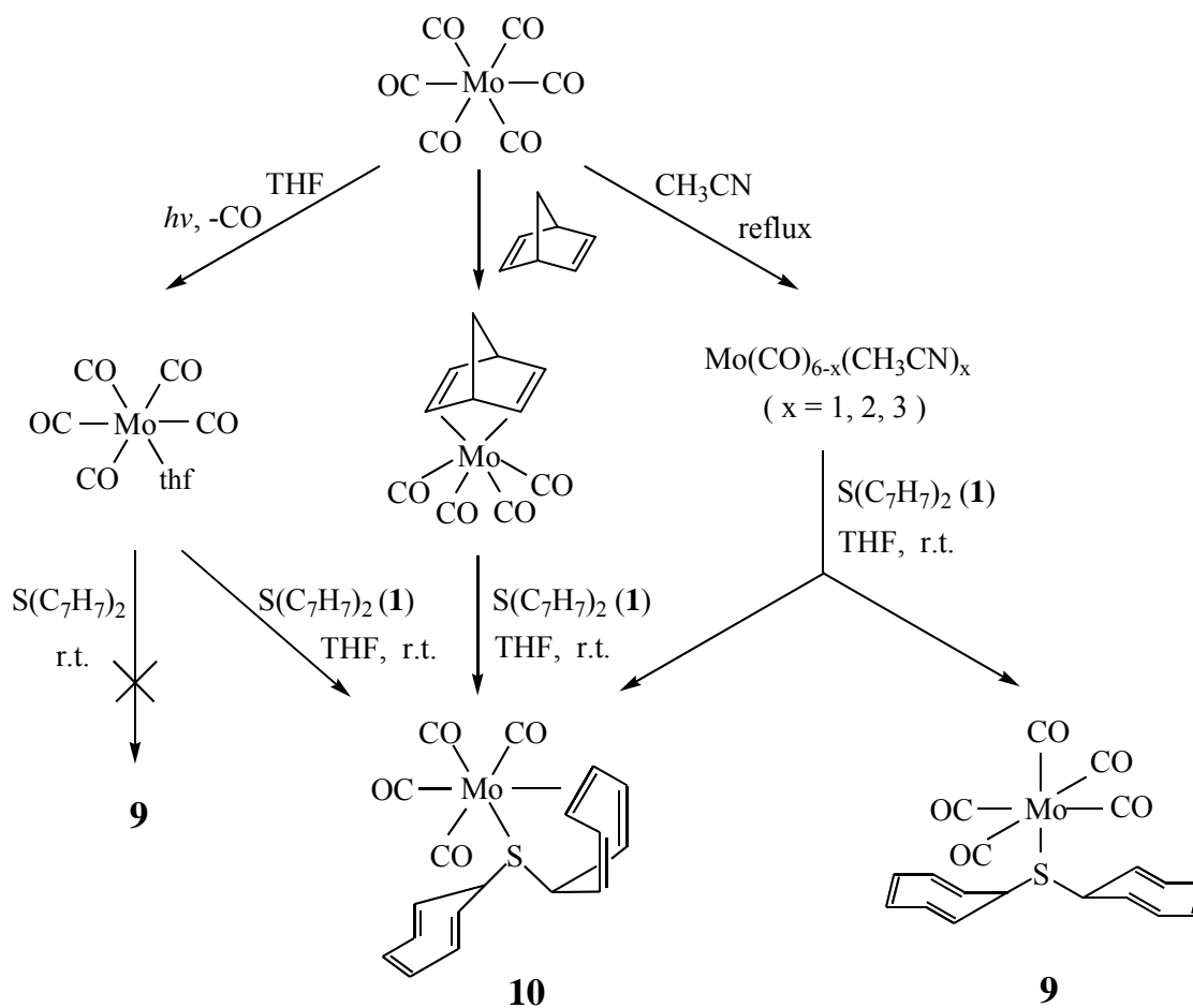
Synthesis of the complexes Mo(CO)_5[S(C_7H_7)_2] ( 9 ) and Mo(CO)_4[(\eta^2-C_7H_7)S(C_7H_7)] ( 10 )
