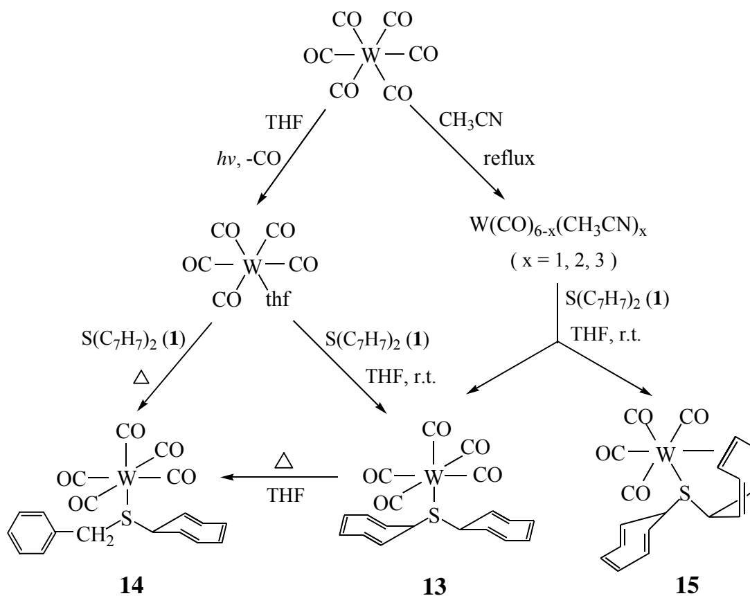
Synthesis of the complexes \text{W}(\text{CO})_5[\text{S}(\text{C}_7\text{H}_7)_2] ( 13 ), \text{W}(\text{CO})_5[\text{PhCH}_2\text{S}(\text{C}_7\text{H}_7)] ( 14 ) and \text{W}(\text{CO})_4[(\eta^2\text{-C}_7\text{H}_7)\text{S}(\text{C}_7\text{H}_7)] ( 15 )
