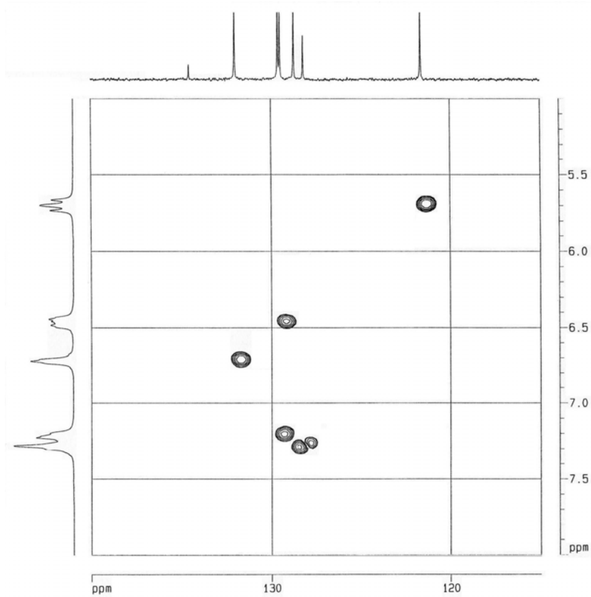
Fig.11. Contour plot of the 2D ^{13}C/^1H HETCOR NMR experiment with complex 7 (in CDCl_3 at 25 °C)
