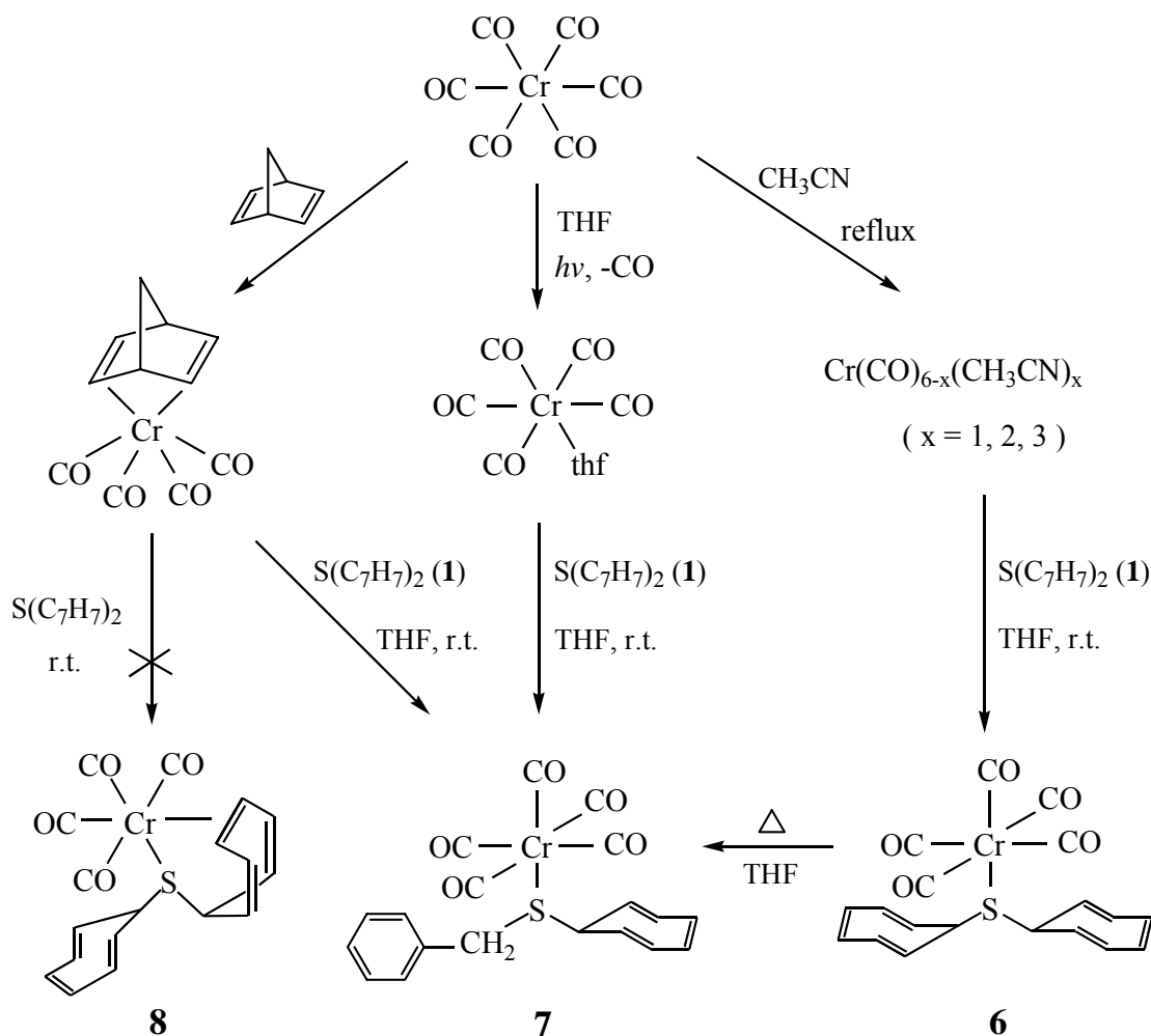
Fig.9. Synthesis of the complexes Cr(CO) 5 [S(C 7 H 7 ) 2 ] (6) and Cr(CO) 5 [PhCH 2 S(C 7 H 7 )] (7)
