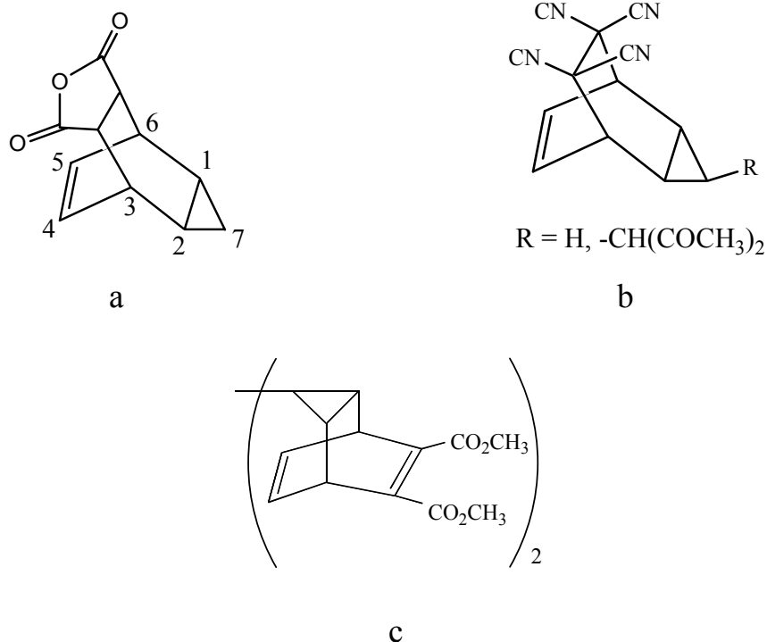
Fig.4. Diels-Alder products reported in earlier work [90-92]
