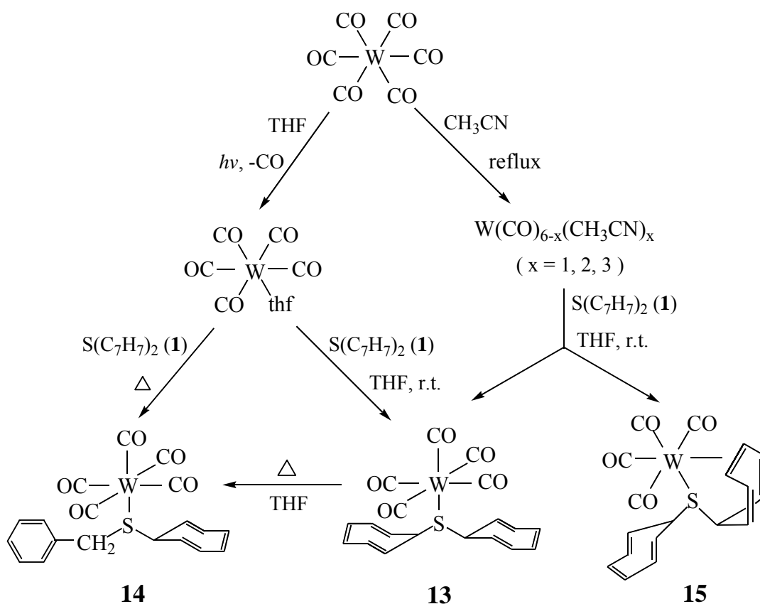
Fig.16. Synthesis of the complexes W(CO) 5 [S(C 7 H 7 ) 2 ] ( 13 ), W(CO) 5 [PhCH 2 S(C 7 H 7 )] ( 14 ) and W(CO) 4 [(η 2 -C 7 H 7 )S(C 7 H 7 )] ( 15 )
