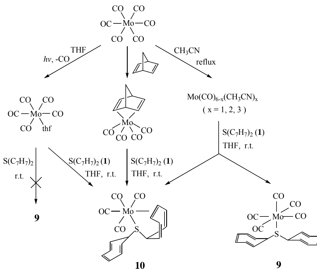
Fig.13. Synthesis of the complexes Mo(CO) 5 [S(C 7 H 7 ) 2 ] ( 9 ) and Mo(CO) 4 [(η 2 -C 7 H 7 )S(C 7 H 7 )] ( 10 )
