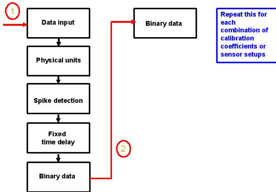
Figure 4: Structure of the programme package TK3, part 1, generation of the physical parameters.
