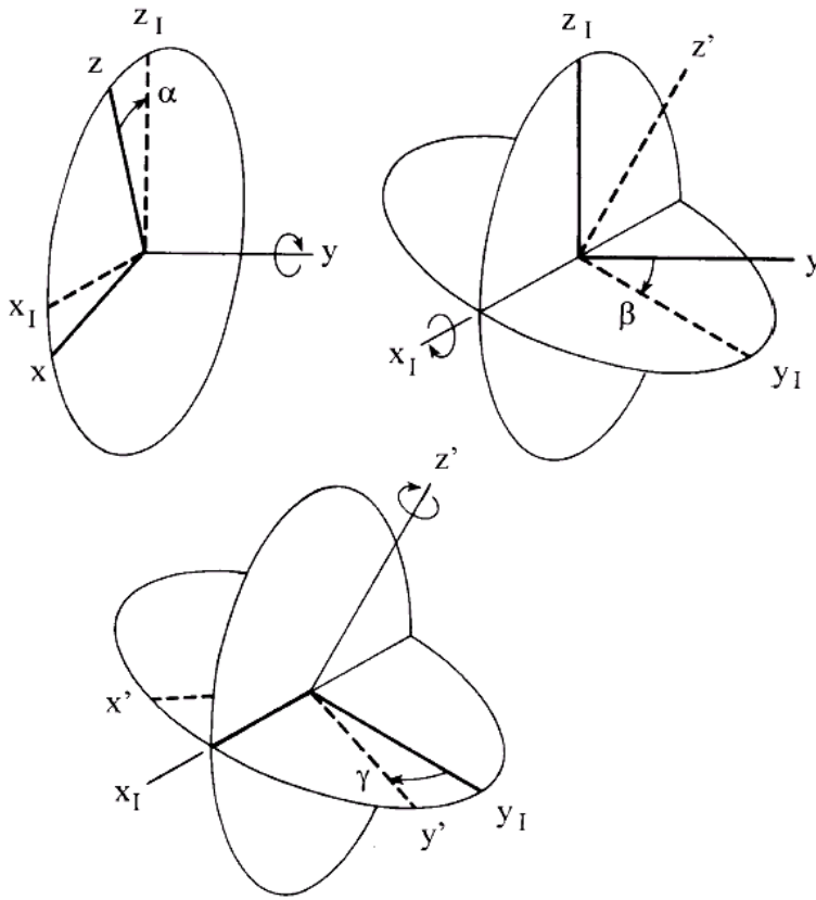
Figure 7: Definition of rotation angles after Wilczak et al. (2001)
