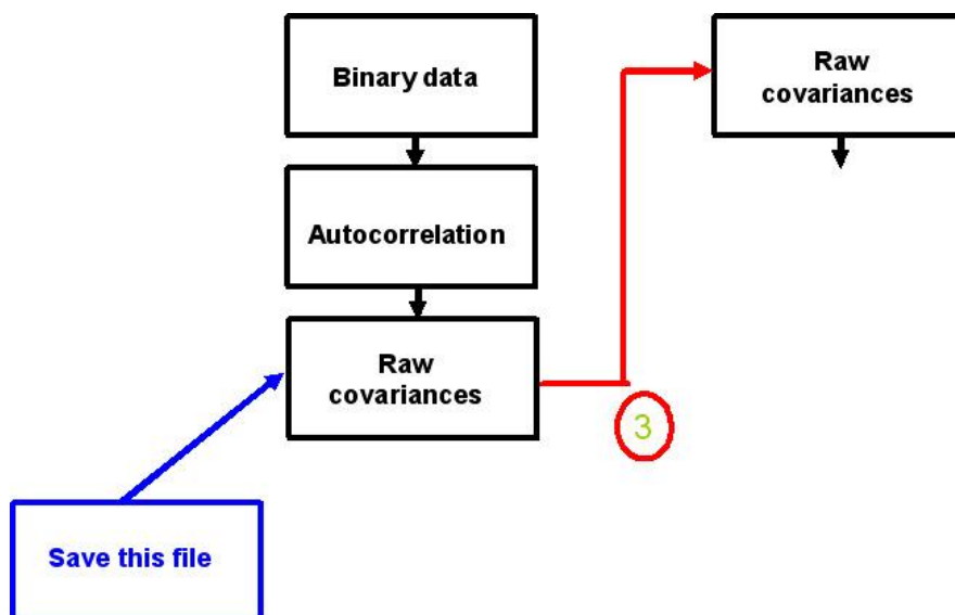
Figure 5: Structure of the programme package TK3, part 2, generation of raw covariances.
