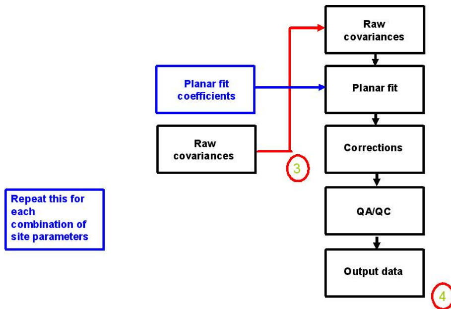
Figure 6: Structure of the programme package TK3, part 3, generation final results.
