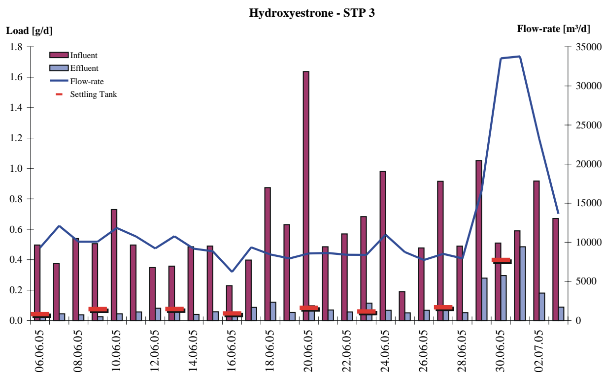
Figure 42: Daily loads of hydroxyestrone in the inflow and the effluent of STP 3 as well as the effluent of the settling tank over the sampling period. Additionally the wastewater flow-rate during the sampling period is presented.
