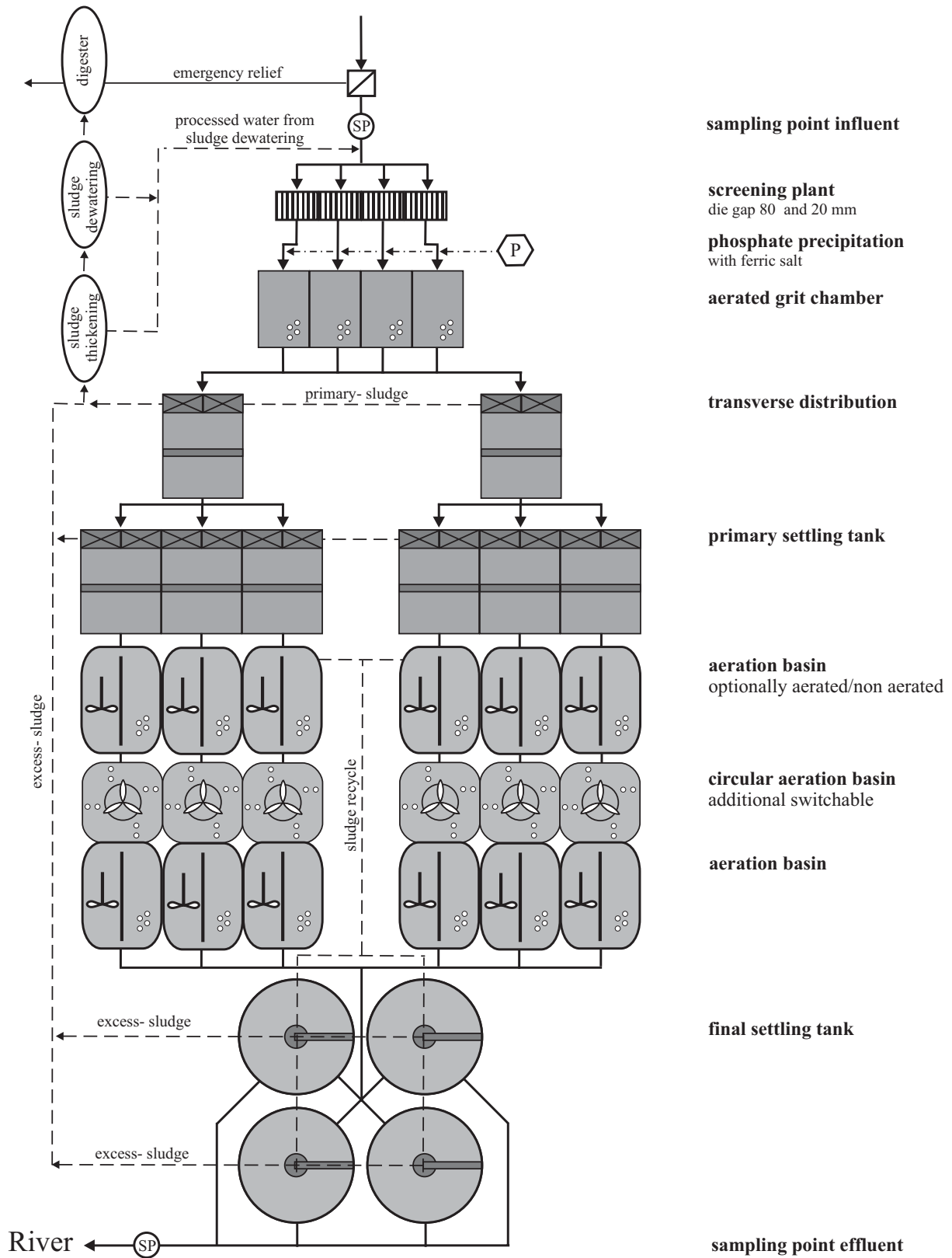
Figure 27: Technical sketch of STP 1 with 250,000 inhabitant equivalent values.
