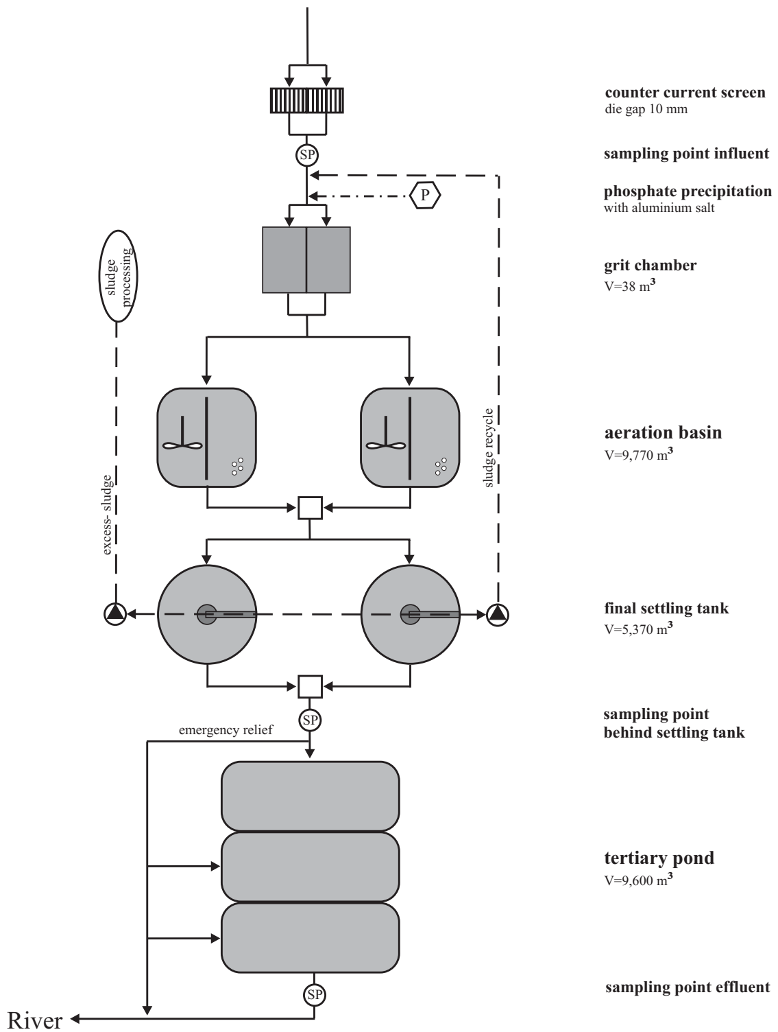
Figure 29: Technical sketch of STP 3 with 32,000 inhabitant equivalent values.
