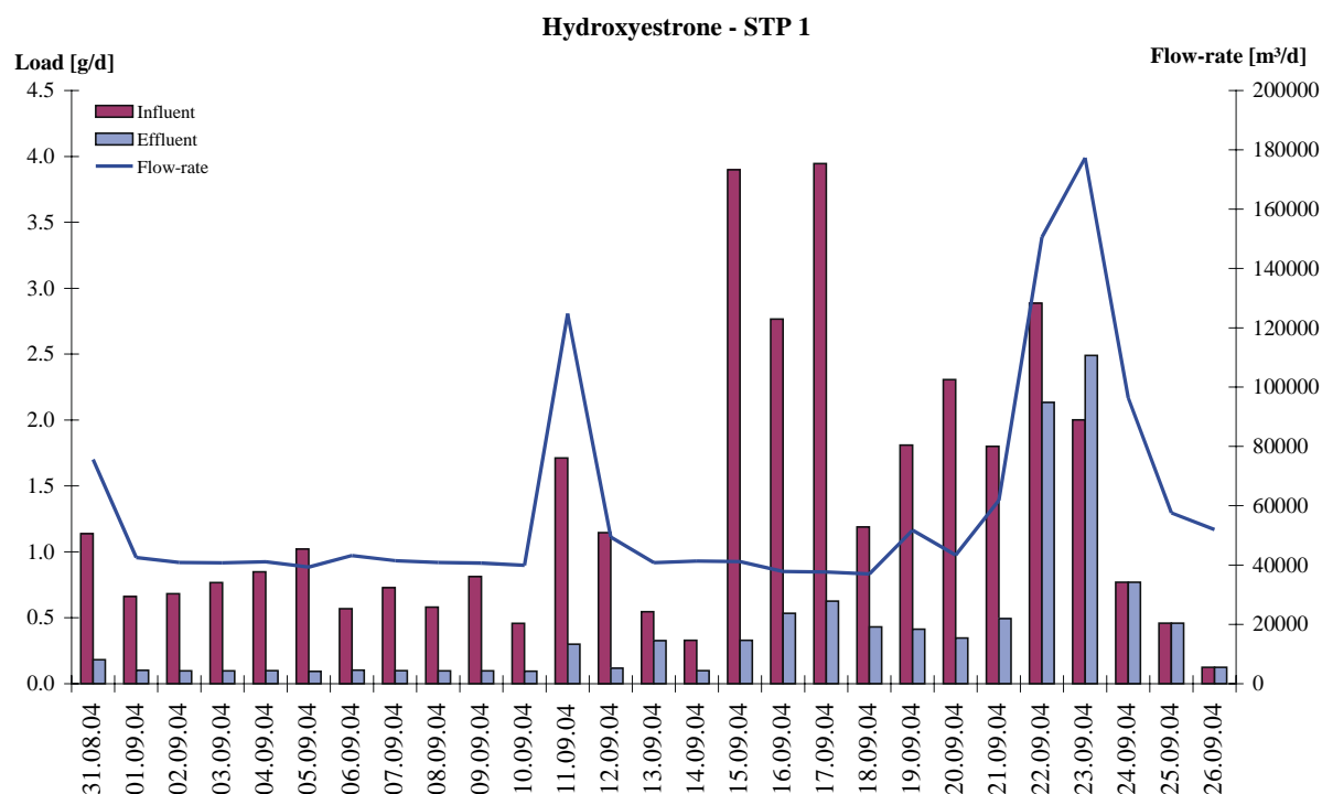
Figure 31: Daily loads of hydroxyestrone in the inflow and the effluent of STP 1 over the sampling period. Additionally the wastewater flow-rate during the sampling period is given.
