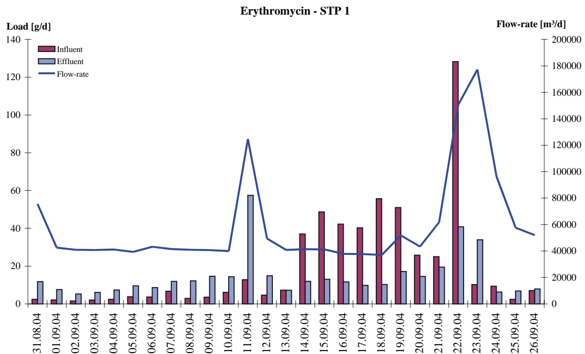
Figure 34: Daily loads of erythromycin in the inflow and the effluent of STP 1 over the sampling period. Additionally the wastewater flow-rate during the sampling period is given.
