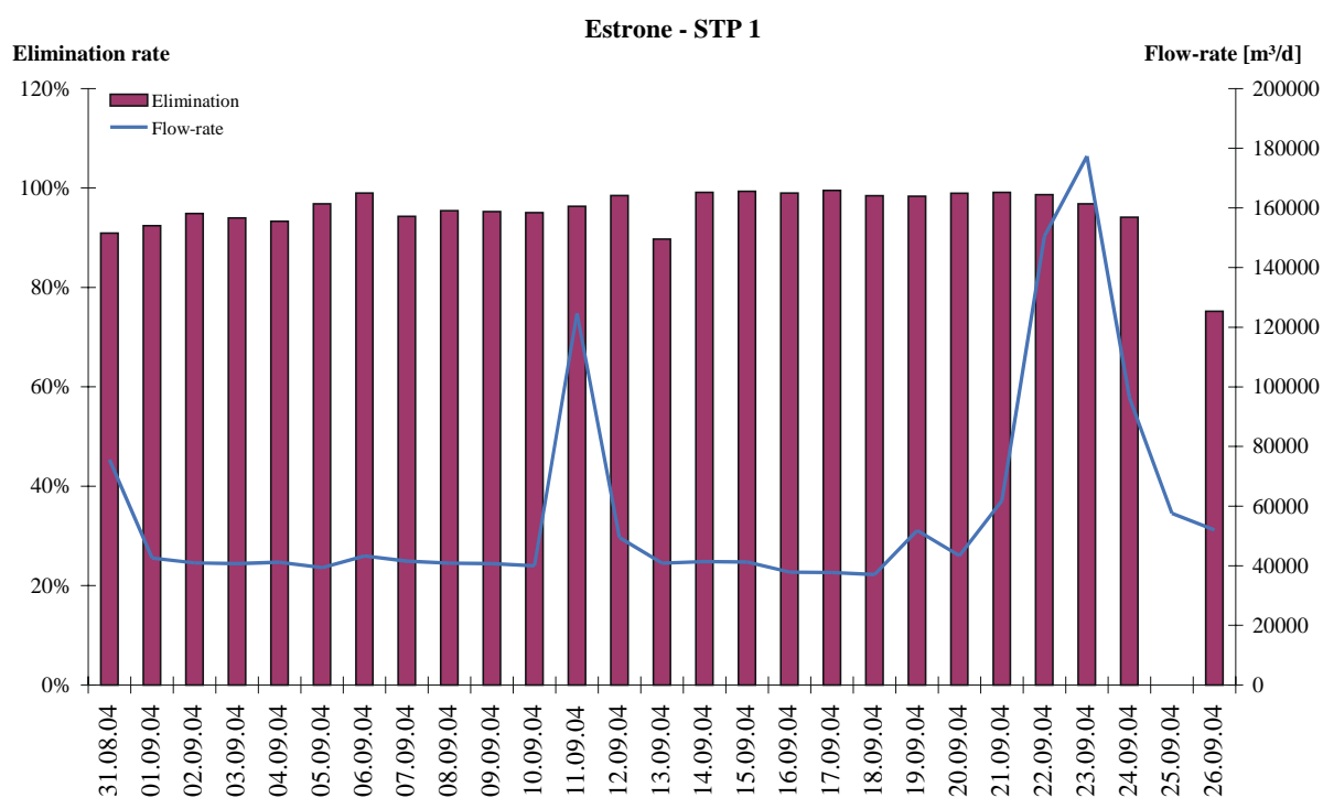
Figure 32: Elimination rates of estrone in STP 1 during the sampling period in comparison to the wastewater flow-rate.
