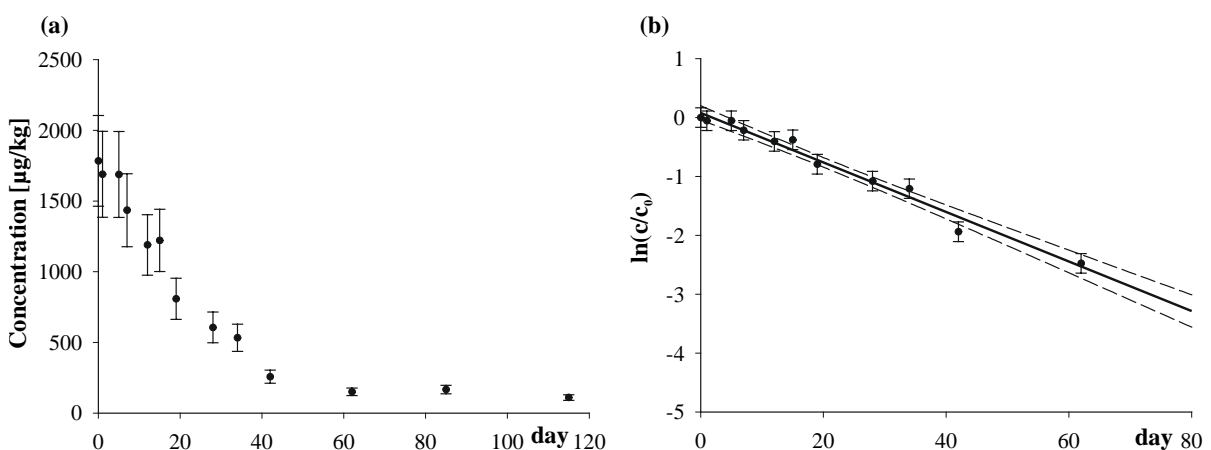
Figure 21: Concentration/time plot of tiamulin during an incubation of 15 single experiments in soil during an incubation of 15 single experiments in soil (a) and plots of the natural logarithm of the concentration/starting concentration ( c/c_0 ) versus time of tiamulin including the 95 % confidence interval. Each point is the average of three extractions of one 110 g batch
