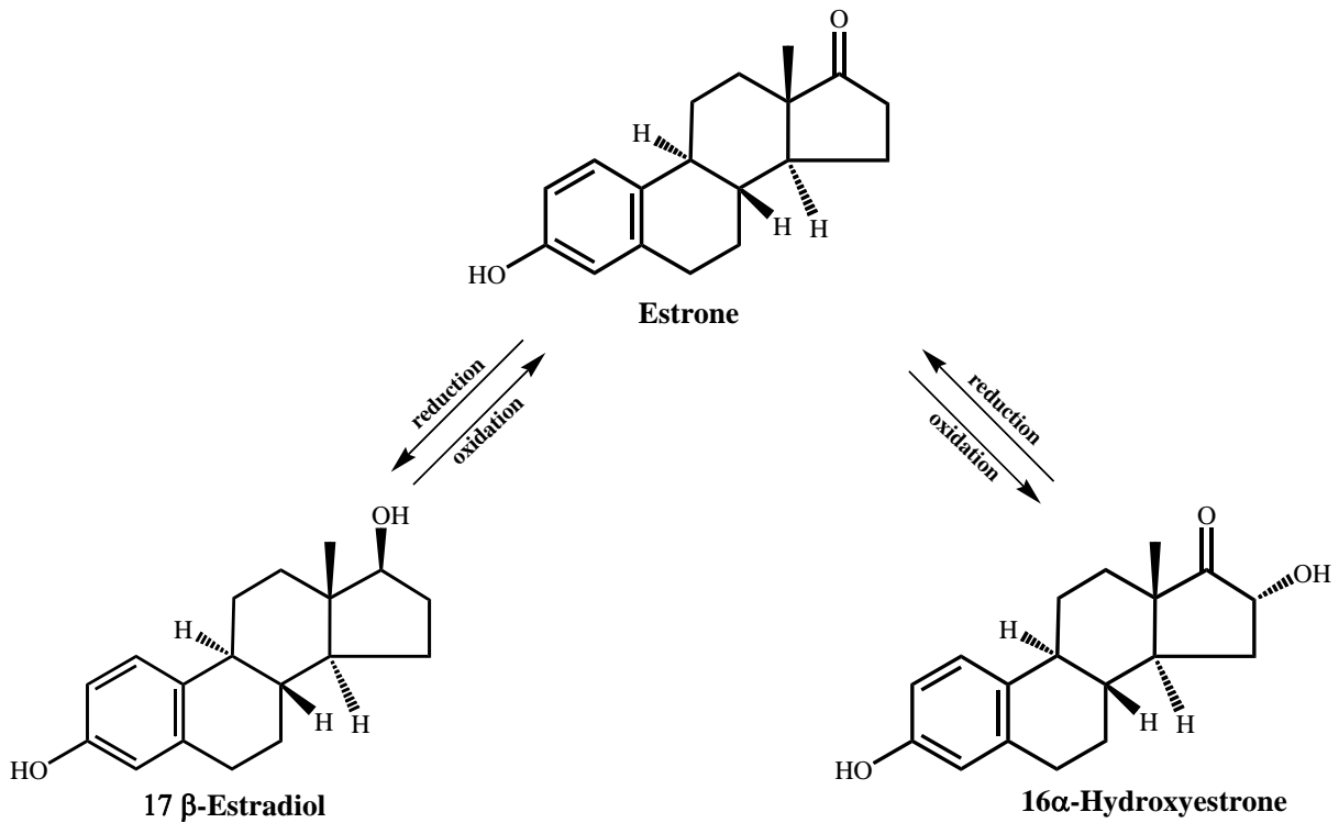
Figure 37: Possible transformation route of hydroxyestrone to estrone and estradiol in STP 2
