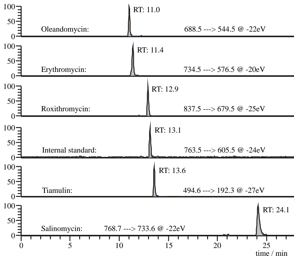
Figure 4: APCI SRM traces of selected macrolides, ionophores and tiamulin for quantification in spiked manure (600 \mu\text{g}/\text{kg} )
