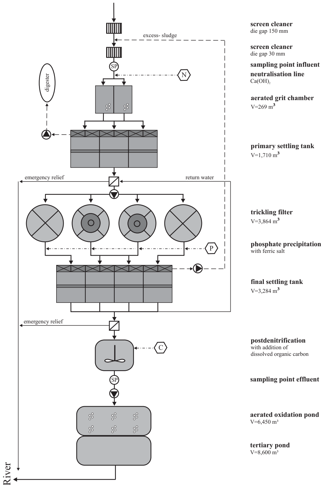
Figure 28: Technical sketch of STP 2 with 64,000 inhabitant equivalent values.
