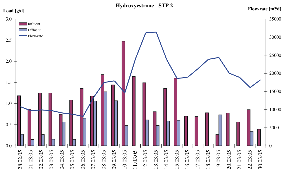
Figure 36: Daily loads of hydroxyestrone in the inflow and the effluent of STP 2 (trickling filter) over the sampling period. Additionally the wastewater flow-rate during the sampling period is presented.
