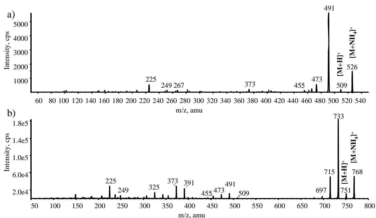
Figure 12: Product ion scan of the ammonia adduct of the metabolite of salinomycin, 526 (a) and product ion scan of the ammonia adduct of salinomycin, 768 (b)
