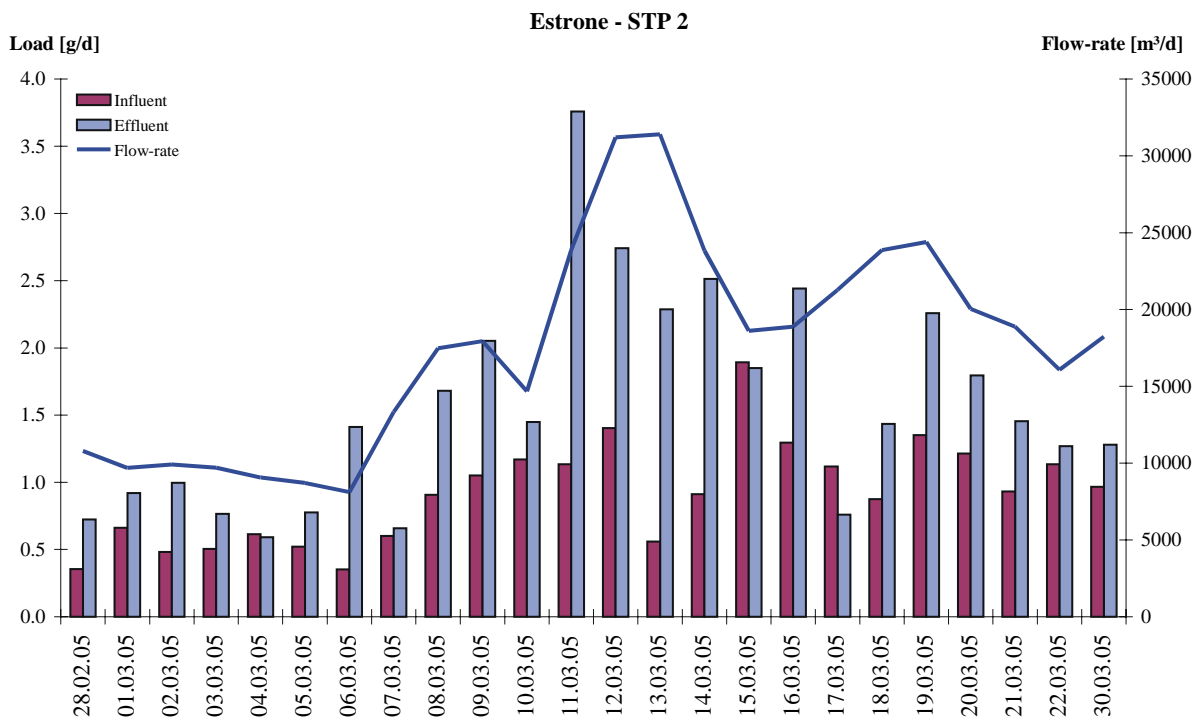
Figure 35: Daily loads of estrone in the inflow and the effluent of STP 2 (trickling filter) over the sampling period. Additionally the wastewater flow-rate during the sampling period is given.
