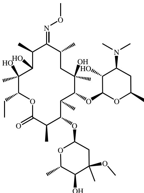
Figure 2: Structural formula of the new internal standard, ( E )-9-[O-(2-methyloxime)]-erythromycin
