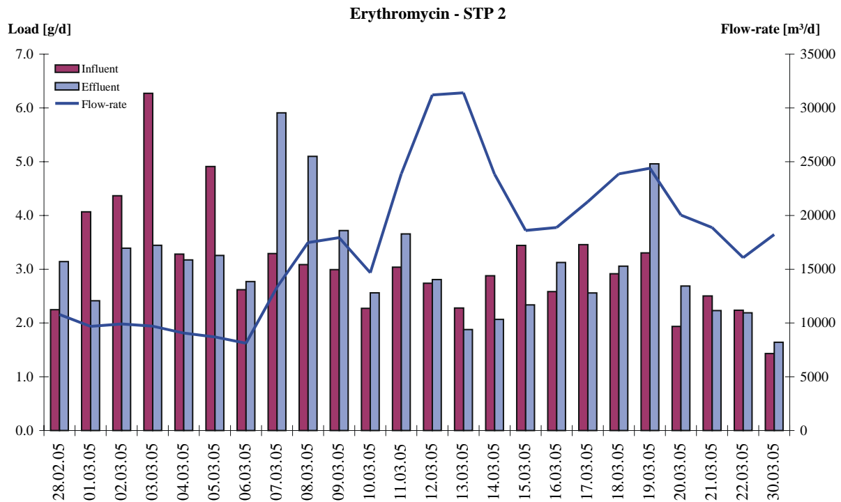
Figure 39: Daily loads of erythromycin as an example for the macrolide antibiotics in the inflow and the effluent of STP 2 (trickling filter) over the sampling period. Additionally the wastewater flow-rate during the sampling period is presented.
