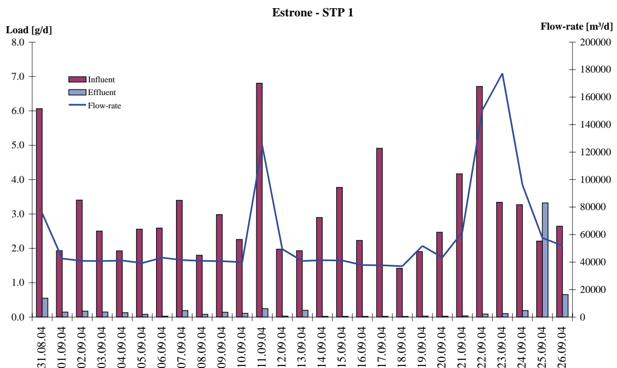
Figure 30: Daily loads of estrone in the inflow and the effluent of STP 1 over the sampling period. Additionally the wastewater flow-rate during the sampling period is given.
