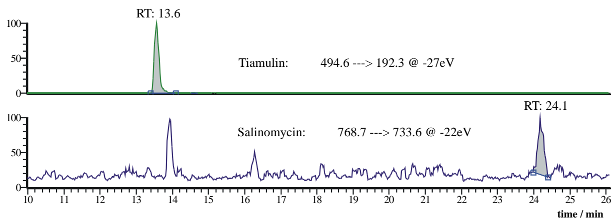
Figure 6: APCI SRM traces of a manure sample from a farm, that applied tiamulin and salinomycin. Tiamulin (43 \mu\text{g}/\text{kg} ) and salinomycin (11 \mu\text{g}/\text{kg} ) were measured.
