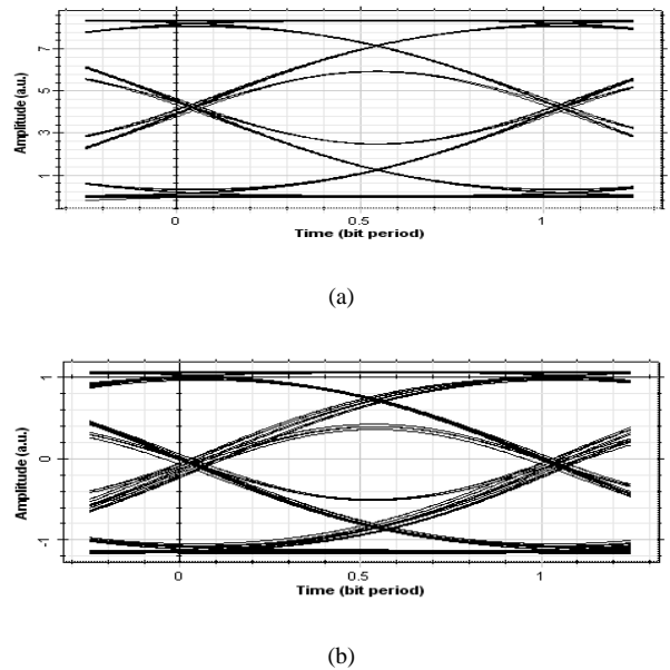
Figure 8: Eye diagram of 900 Mbit/s ASK modulated signal with 10 GHz carrier over 50 km length of single mode fibre: (a) ARoF system, (b) DRoF system.
