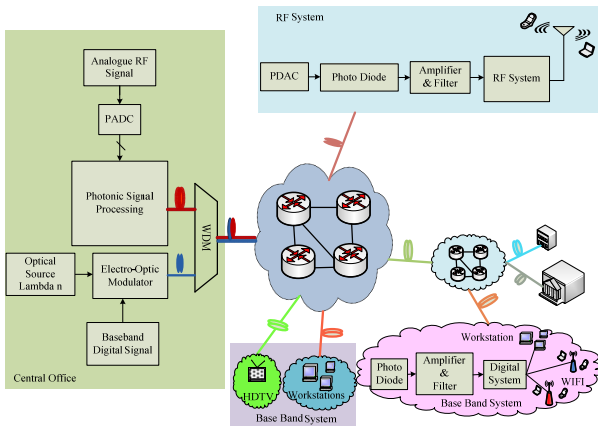
Figure 1: The proposed downlink DRoF system.
