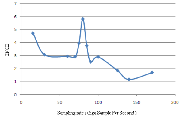
Figure 5: ENOB variation versus sampling rate.
