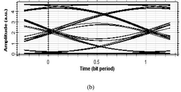
Figure 7: Eye diagram of 900 Mbit/s ASK modulated signal with 10 GHz carrier over 35 km length of single-mode fibre: (a) ARoF system, (b) DRoF system.
