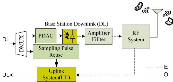
Figure 3: The Base-Station System that uses PDAC.
