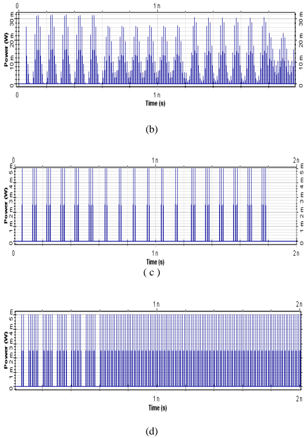
Figure 6: (a), A sample 64 QAM, 10 GHz RF signal, (b) Sampled optical signal, (c), Optical signal of MSB, (d) Optical signal of LSB.
