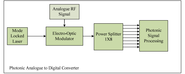
Figure 2: The photonic ADC's architecture.
