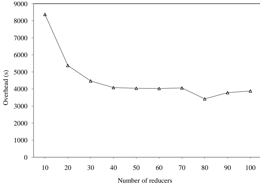
Figure 4.13: The impact of reducers.
