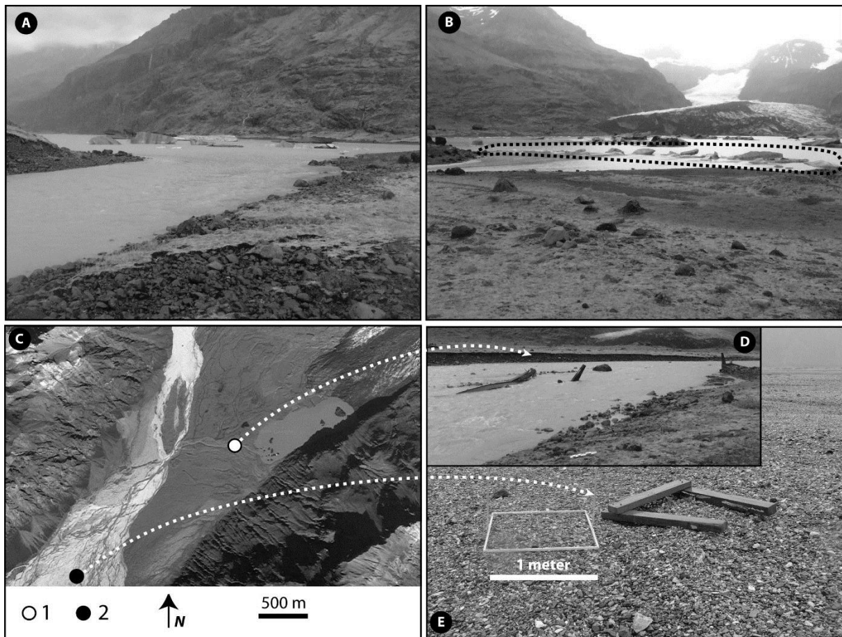
Figure 3 - Formation of icebergs jam and impact of the 2006 icebergs jam flood downstream of the Morsárjökull proglacial lake. A: icebergs accumulation at the outlet of the ice-contact lake. B: formation of the icebergs jam. C: Positions of the bridge destroyed during the 2006 icebergs jam flood. 1: pre-flood position of the bridge. 2: Position of bridge fragments found in July 2006 after the icebergs jam flood. E: Fragment of the bridge found on the active sandur in July 2006.
