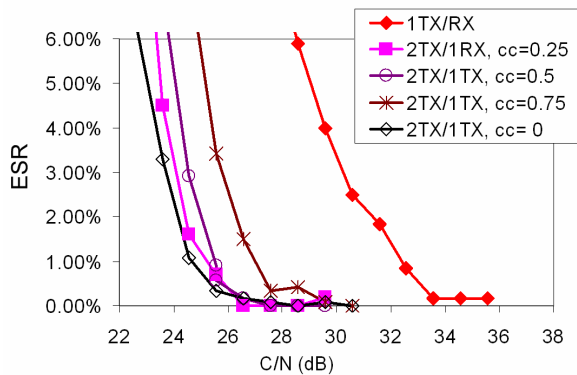
Fig. 5. ESR vs. C/N for indoor channel, UK mode \delta = 1\mu s , F_d = 1\text{ Hz}
