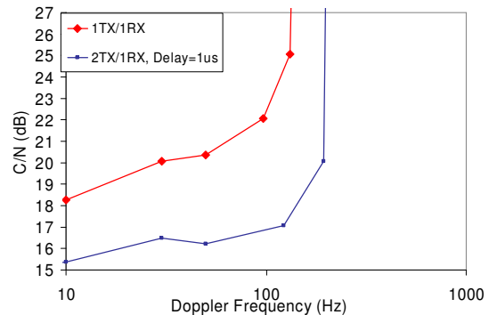
Fig. 7. C/N at TOV vs. Doppler Frequency, TU, 4-QAM UK mode, ESR= 5%, \rho = 0.25 , \delta = 1\mu s
