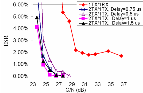
Fig. 6. ESR vs. C/N for TU channel, UK mode, \rho = 0.25 , F_d = 50\text{ Hz}
