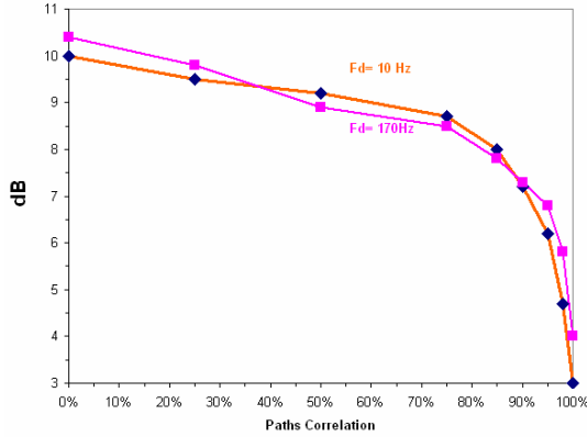
Fig. 8. Dibcom SIMO Receive Diversity Gain for different Channel Cross Correlations (2K, QPSK \frac{3}{4} , \frac{1}{32} ) for a TU6 Channel at low and high Doppler.
