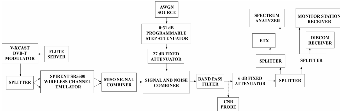
Fig. 2. Block diagram of laboratory test bench
