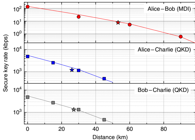
Fig. 3 Secure key rates vs. distance. MDI-QKD (top diagram) and QKD (centre and bottom diagrams) secure key rates for a Z ( X ) basis probability equal to 80% (20%) and a security parameter e_{\text{sec}} \lesssim 10^{-10} are shown as a function of distance. Because the reconfigurable scheme is symmetrically deployed, the distance between Alice and Bob (top) is approximately twice the distance between Alice and Charlie (centre) and Bob and Charlie (bottom). All the distances have been calculated assuming 0.2 dB/km attenuation on the channel, except for the data points indicated by stars, where a real fibre was used. The projected time to attain the shown key rates is 25 h of which 3 min are spent on QKD and the rest on MDI-QKD, to balance their key rates. The fitting lines are the result of a numerical simulation with the parameters mentioned above and the following additional ones: Charlie’s insertion loss, 1.1 dB; detectors’ efficiency and temperature, 20% and 0^\circ , respectively; afterpulsing, 4%; dark count probability per gate, 1.6 \times 10^{-5} ; error correction coefficient, 1.16
