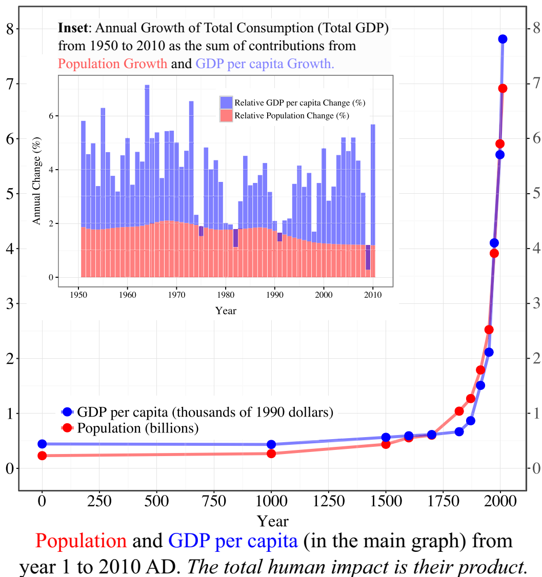
Figure 1. World population and GDP per capita from year 1 to 2010 AD. The total human impact is their product. The inset shows the relative annual change of each between 1950 and 2010 [228–230]. Their averages were 1.69% and 2.21%, respectively, out of a total of ~4% (average annual change in GDP). Therefore, growth in population and consumption per capita have both played comparably important roles in the remarkable increase of human impact on planet Earth. This ~4% total growth corresponds to doubling the total impact every ~17 years. Note that the contribution from population growth has been relatively steady, while the contribution from the relative change in GDP per capita has been much more variable from year to year (even negative for some years). See Footnote 2 for a description of the mathematical formula used to generate the inset and sources of data.
