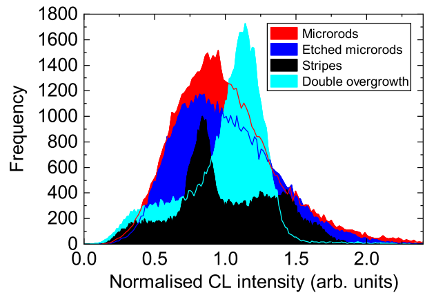
Figure 3. Histogram of the intensities from the CL intensity images of the GaN NBE emission in Fig. 2(e)–(h). The intensities are normalised using their respective mean intensity for comparison.
