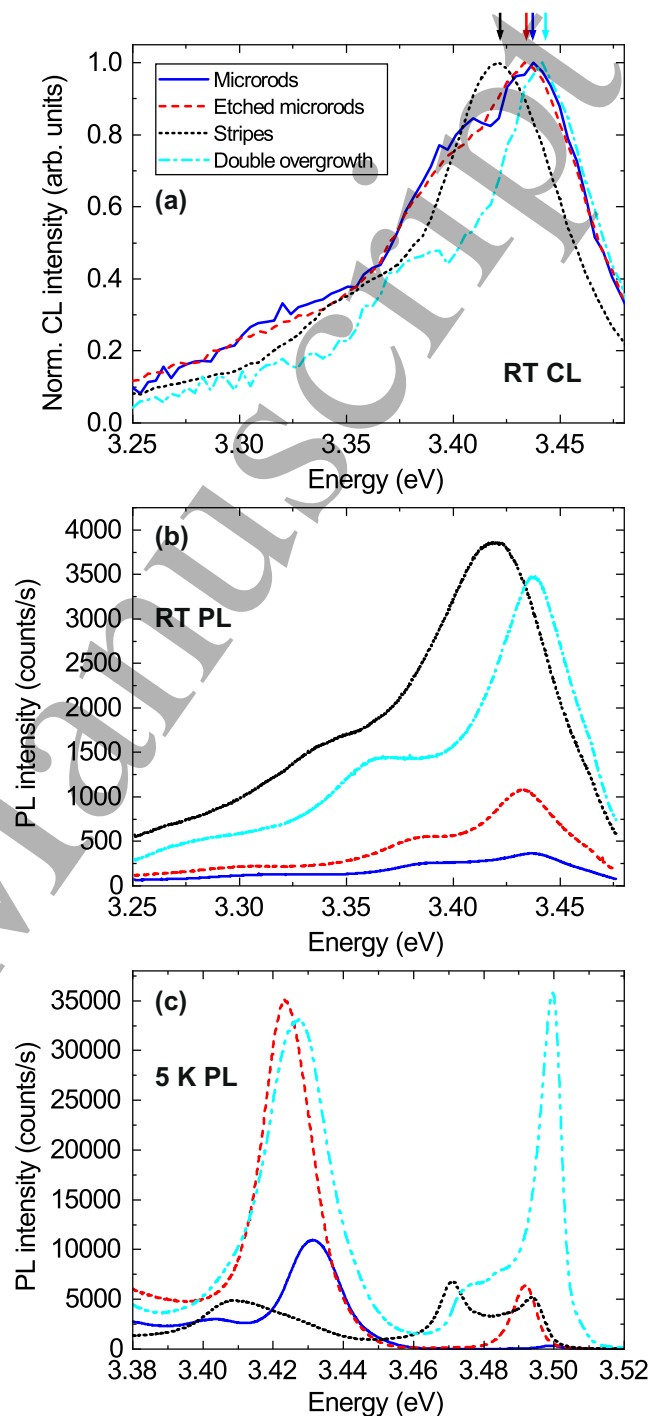
Figure 4. Luminescence spectra of the four different overgrown microstructures: (a) RT CL spectra normalised to the GaN NBE emission. The CL spectra were generated from the hyperspectral data set also used for generating the GaN NBE intensity images in Fig. 2(e)–(h). The approximate position of the NBE peak is marked by arrows. PL spectra at (b) RT and (c) low temperature (5 K).
