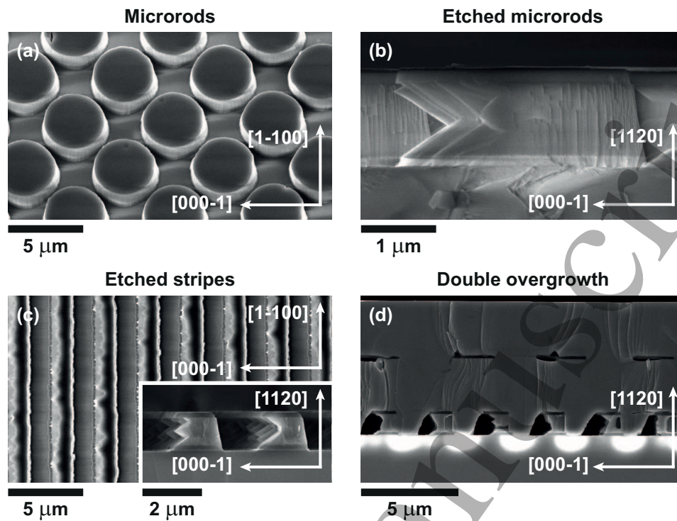
Figure 1. SE images of the four different GaN microstructures before overgrowth (except (d)): (a) top-view of regular microrod array ( 4\ \mu\text{m} diameter and pitch), (b) cross-section of etched microrod array in mushroom configuration ( 2.5\ \mu\text{m} diameter and pitch), (c) top-view and cross-section (inset) of etched stripes ( 1.5\ \mu\text{m} strip and gap width) and (d) cross-section of the double overgrowth sample after the entire growth using etched stripes ( 2.5\ \mu\text{m} diameter and pitch) followed by etched microrods ( 1.5\ \mu\text{m} stripe and gap width). The darker layers in the cross-section images are parts of the \text{SiO}_2 mask.
