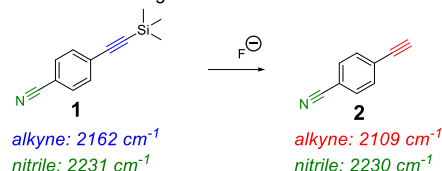
Figure 1 Previous reports of sensing and quantification using alkyne-tag Raman imaging. (i) A previous example of an irreversible sensor for hydrogen sulfide (H 2 S) detection 11 and (ii) a reversible sensor for quantifying intracellular pH. 12 This work reports an extremely low molecular weight Raman sensor ( 1 ) for ratiometric detection of fluoride ions.
