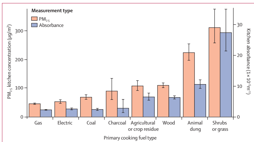
Figure 2: Summary of PM_{2.5} kitchen concentrations ( \mu\text{g}/\text{m}^3 ) and absorbance levels ( 1 \times 10^{-5} \text{m}^{-1} ) by primary fuel type. Error bars are 95% CIs. Point estimates are geometric means.
