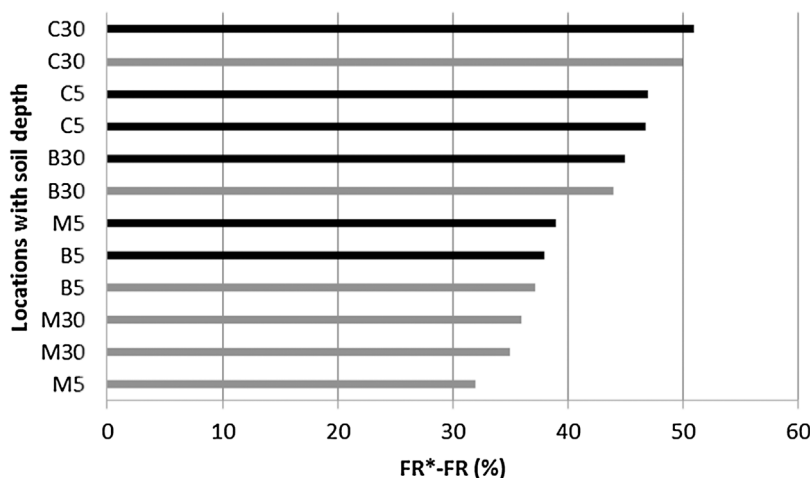
Fig. 6. The difference between the FR^* - FR for all sites and soil profiles for SPI. The positive values indicate that drought indices are more reliable than the hydraulic model due to the uncertainties of the model. Black and grey bars indicate the highest sensitive and median sensitive values of perturbed model respectively. Values of FAR^* - FAR are the same as FR^* - FR . FR^* represents the mean of three assessed parameters ( \theta_r , \theta_s , \alpha ). B: Bourke, C: Cairns, M: Melbourne.
