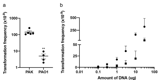
Fig. 4. P. aeruginosa is capable of natural transformation of plasmid DNA in static broth cultures. Carbenicillin-resistant transformants obtained from static broth cultures incubated at 37 °C for 24 h with (a) 10 µg pUCPSK or (b) 0.1–30 µg pUCPSK with PAK (circles) or PAO1 (squares). The mean of each set of technical triplicates was calculated to give an n \geq 3 , which is presented as mean±SEM. For (a) ** P < 0.005 ; Mann–Whitney U -test compared to PAK. For (b) there was no significant difference ( P > 0.05 ; Friedman with Dunn’s multiple comparisons test) between DNA concentrations (0.1–30 µg) for both strains.
