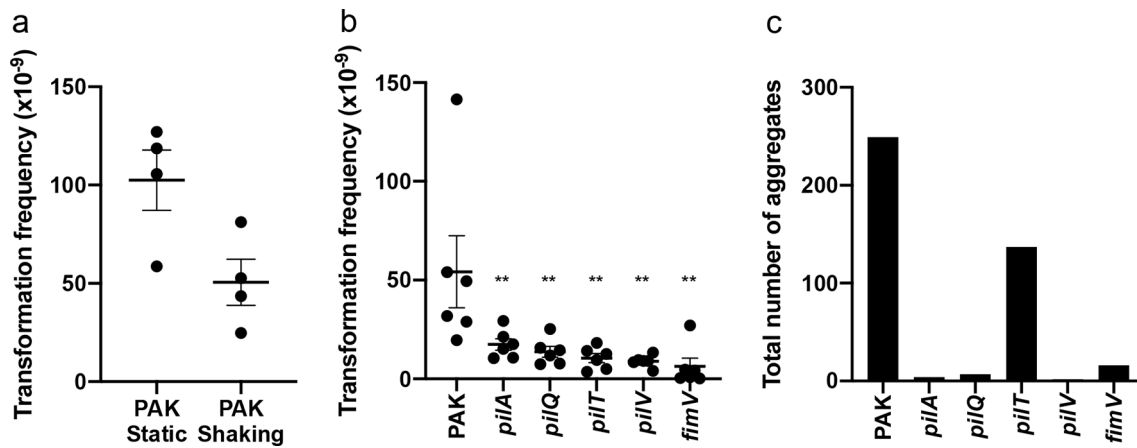
Fig. 5. T4P are not absolutely required for natural transformation. Static (a–c) or shaking (a) broth cultures were incubated at 37 °C for 24 h with 10 µg pUCPSK and the number of (a, b) carbenicillin-resistant transformants or (c) aggregates determined. For (a, b) the mean of each set of technical triplicates was calculated to give an n \geq 3 , which is presented as mean \pm SEM. For (a) P > 0.05 (ns); Mann–Whitney U -test. For (b) ** P < 0.005 ; Mann–Whitney U -test compared to PAK. For (c) the total number of aggregates from 60 random fields imaged on 3 separate days (20 fields/day) is presented.
