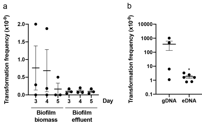
Fig. 1. P. aeruginosa is capable of natural transformation in continuous-flow biofilms. Carbenicillin- or gentamicin-resistant transformants obtained from continuous-flow biofilms of PAO1 in Tygon tubing. For (a) pUCPSK (Carb R ) was added to the media influent (at a final concentration of 1 µg ml -1 with flow rate of 80 µg min -1 ) with either the biofilm biomass or effluent harvested and plated on carbenicillin selective agar plates on the indicated day. For (b) sterile gDNA or total eDNA obtained from PAO1 GFP (Gm R ) (at a final concentration of 0.1 mg ml -1 with flow rate of 80 µg min -1 ) was added to the media influent and the biofilm biomass harvested and plated on gentamicin selective agar plates after 5 days. The mean of each set of technical triplicates was calculated to give an n \geq 4 , which is presented as mean ± SEM (* P < 0.05 ; Mann–Whitney U -test compared to gDNA).
