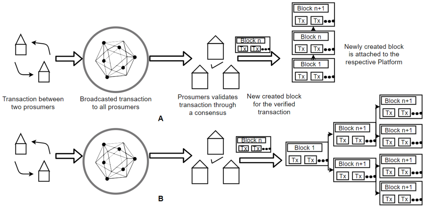
Fig. 3. The process of creating a block and attaching to the respective platform: A for blockchain; B for directed acrylic graph.
