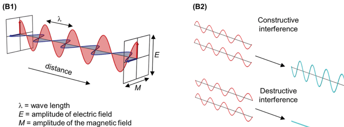
Figures B1 and B2. Property of light and constructive interference
