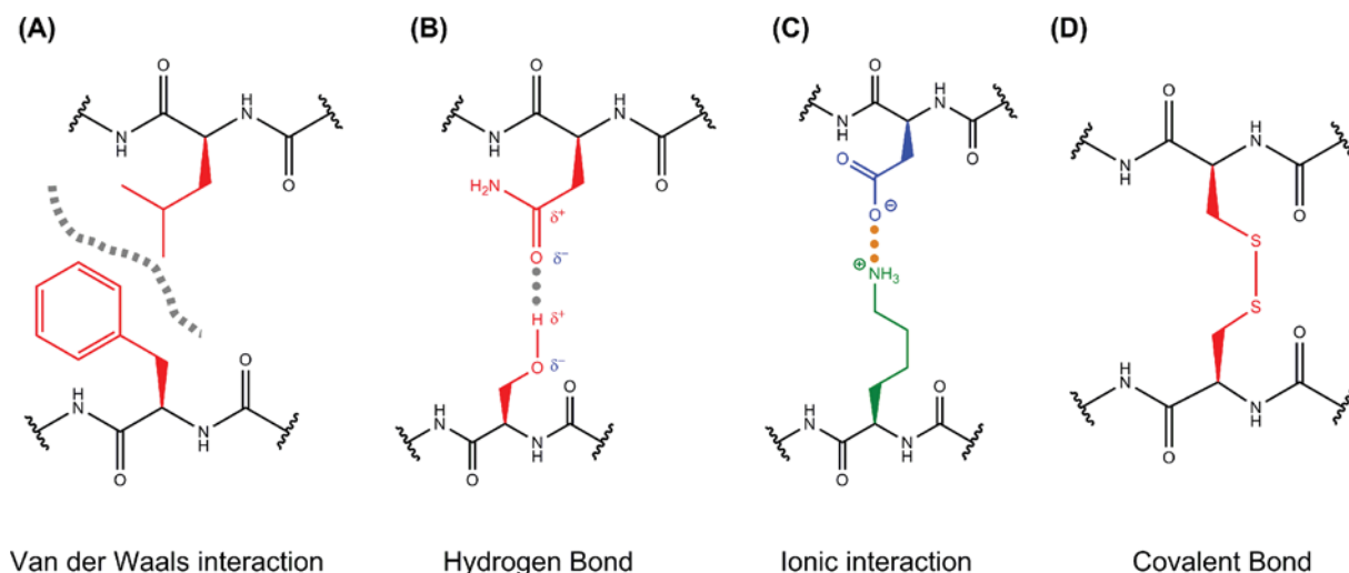
Figure 2. Intermolecular interactions
