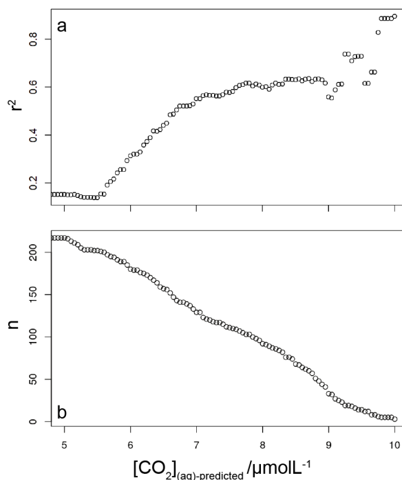
Figure 6. Pearson correlation coefficient (panel a) of a reducing sample of all compiled \text{CO}_{2(\varepsilon_p-\text{alk})} (Table 1) vs the time-equivalent estimate from ice core records (Bereiter et al. (2015); Table 2). The sample reduces stepwise by 0.05 \mu\text{molL}^{-1} , and the number of records in each subsample is shown in panel b.
