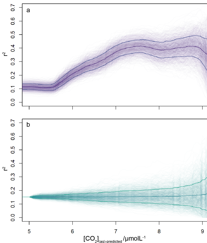
Figure 8. Pearson correlation coefficient of a reducing sample of all compiled \text{CO}_{2(\varepsilon_p-\text{alk})} (Table 1) vs the time-equivalent estimate from ice core records (Bereiter et al. (2015); Table 2). As in Figure 6 the sample reduces stepwise by 0.05 \mu\text{molL}^{-1} . Panel a shows a 1000 member Monte Carlo analysis, whereby uncertainty in \text{CO}_{2(\varepsilon_p-\text{alk})} and age is considered, as detailed in the text. Panel b shows a similar 1000 member Monte Carlo analysis, but with random sampling of the whole \text{CO}_{2(\varepsilon_p-\text{alk})} population so that the number of samples is equivalent to the dataset shown in panel a, ie the size of the sample follows that shown in Figure 6b. Means and one \sigma uncertainties are shown as the bold lines.
