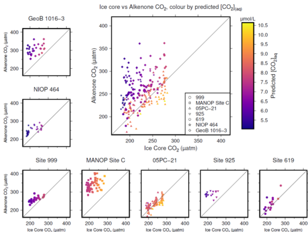
Figure 4. Crossplots of \text{CO}_2(\epsilon_p\text{-alk}) -based atmospheric \text{CO}_2 (y-axes vs Bereiter et al. (2015); Table 2)). The large panel compiles all sites, with the exception of MANOP Site C, as explained in the text. Symbols are coloured by predicted [\text{CO}_2]_{\text{aq}} for each site and time as explained in the text. Full sources for alkenone data are shown in Table 1. A 1:1 line is included in all plots for comparison.
