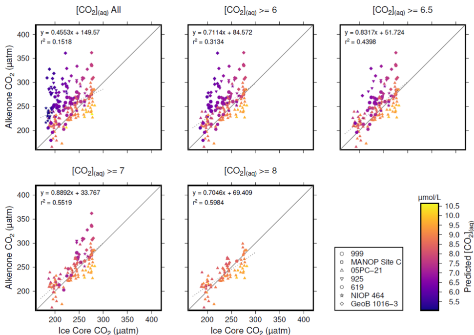
Figure 5. Crossplots of \text{CO}_2(\varepsilon_p\text{-alk}) -based atmospheric \text{CO}_2 (Table 1; y-axes) vs the time-equivalent estimate from ice core records (x-axes; Bereiter et al. (2015); Table 2)). The sample of published values of \text{CO}_2(\varepsilon_p\text{-alk}) was progressively restricted by [\text{CO}_2]_{(\text{aq})\text{-predicted}} , indicated by the subplot titles. Individual values are coloured by [\text{CO}_2]_{(\text{aq})\text{-predicted}} , and Sites indicated by shape (see key). Pearson correlation coefficients and equations of best fit are shown in each panel, along with a 1:1 line.
