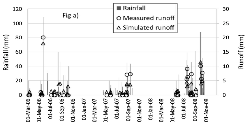
Fig. 7. Comparison between measured (circle) and simulated (triangle) runoff on daily time scale along with rainfall (vertical line) during 2006–08.
