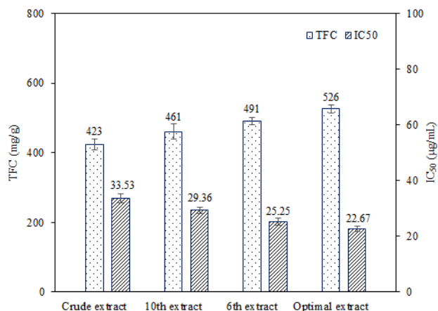
Fig. 5. Effect of TFC on the α-glucosidase inhibition of the plant extract.
