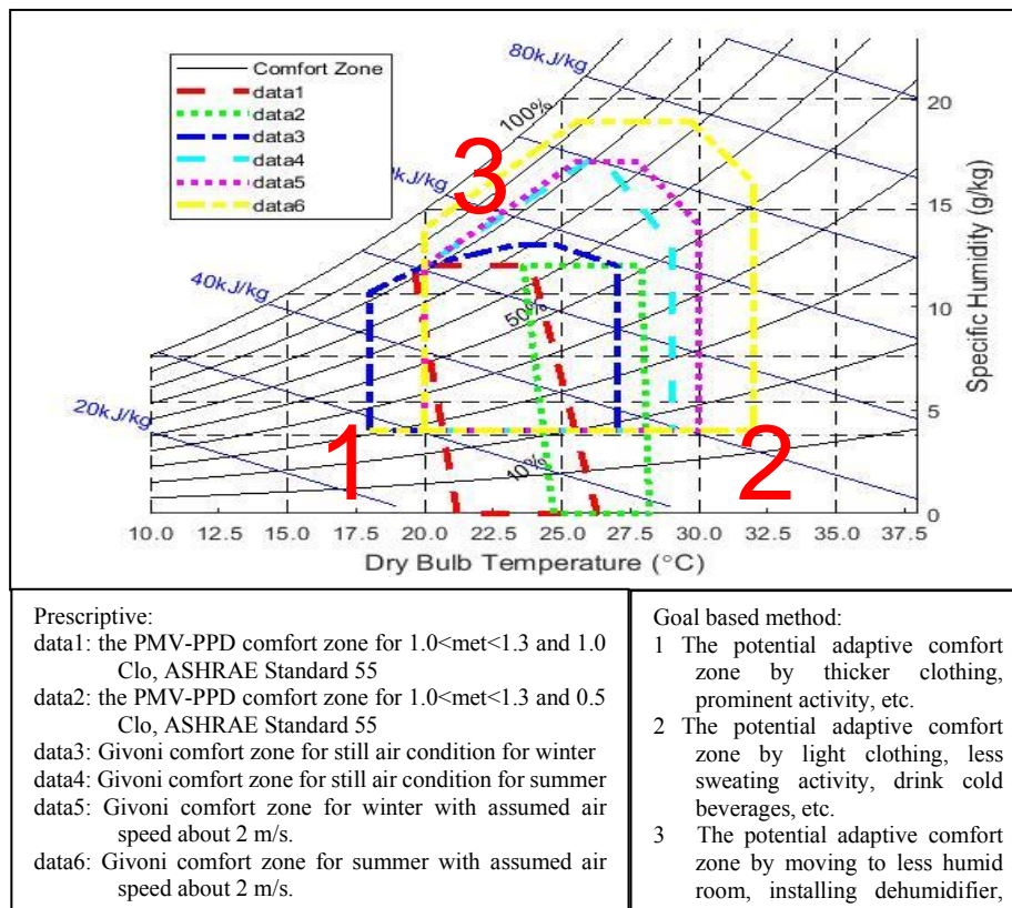
Figure 5. Psychometrics chart showing the comfort zone (PMV-PPD [44]) and Givoni [45]) and potential adaptive comfort zone.
